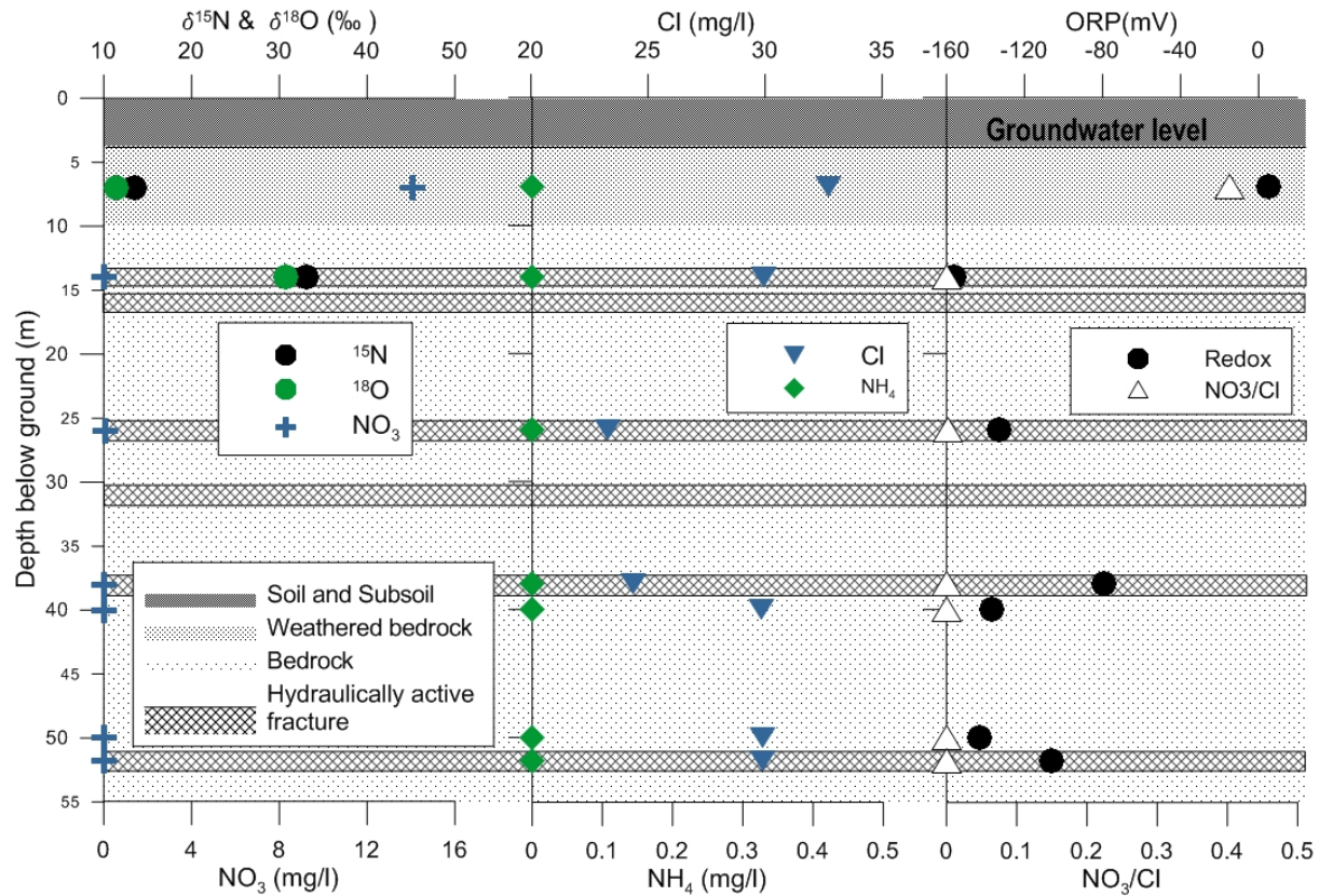
Figure 6 Variation of \text{NO}_3 , \text{NH}_4 , and ORP concentrations and \text{NO}_3 isotope ( \delta^{15}\text{N} and \delta^{18}\text{O} ) values with depth in BH6 cluster, sampled using a packer system and low flow pump.
