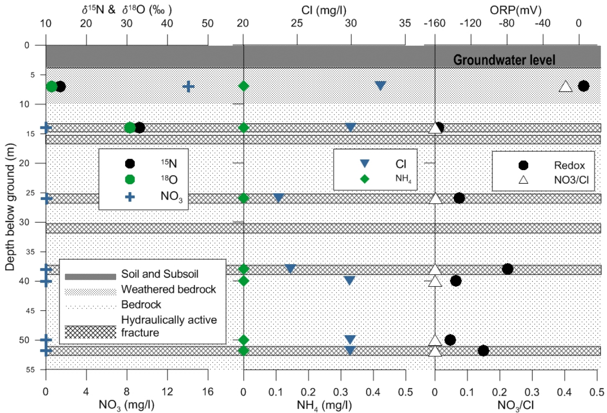
9 Figure 6 Variation of NO 3 - , NH 4 + , and ORP concentrations and NO 3 - isotope ( \delta^{15}\text{N} and \delta^{18}\text{O} ) values with 10 depth in BH6 cluster, sampled using a packer system and low flow pump.
