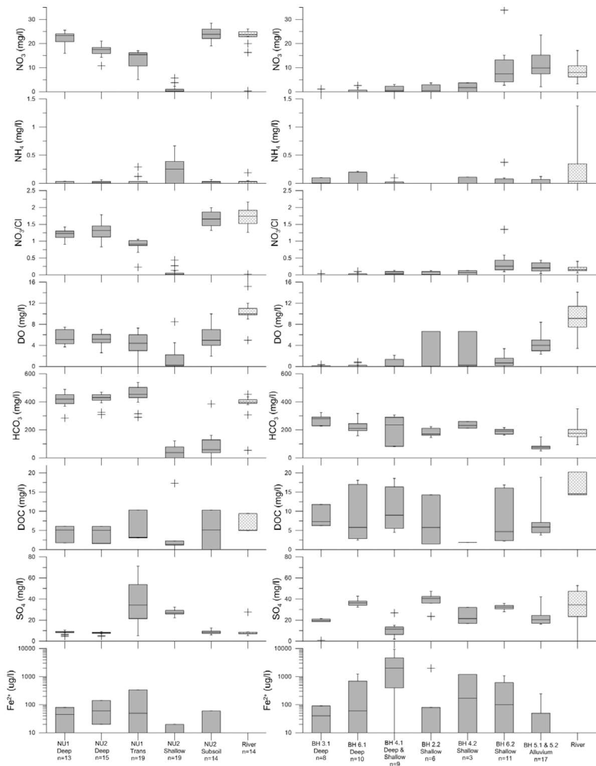
Figure 3 Box and whisker plots of NO 3 , NH 4 , NO 3 /Cl, DO, HCO 3 , DOC, SO 4 and Fe 2+ concentrations in groundwater pathways and rivers in the Nuenna and Glen Burn catchments.
