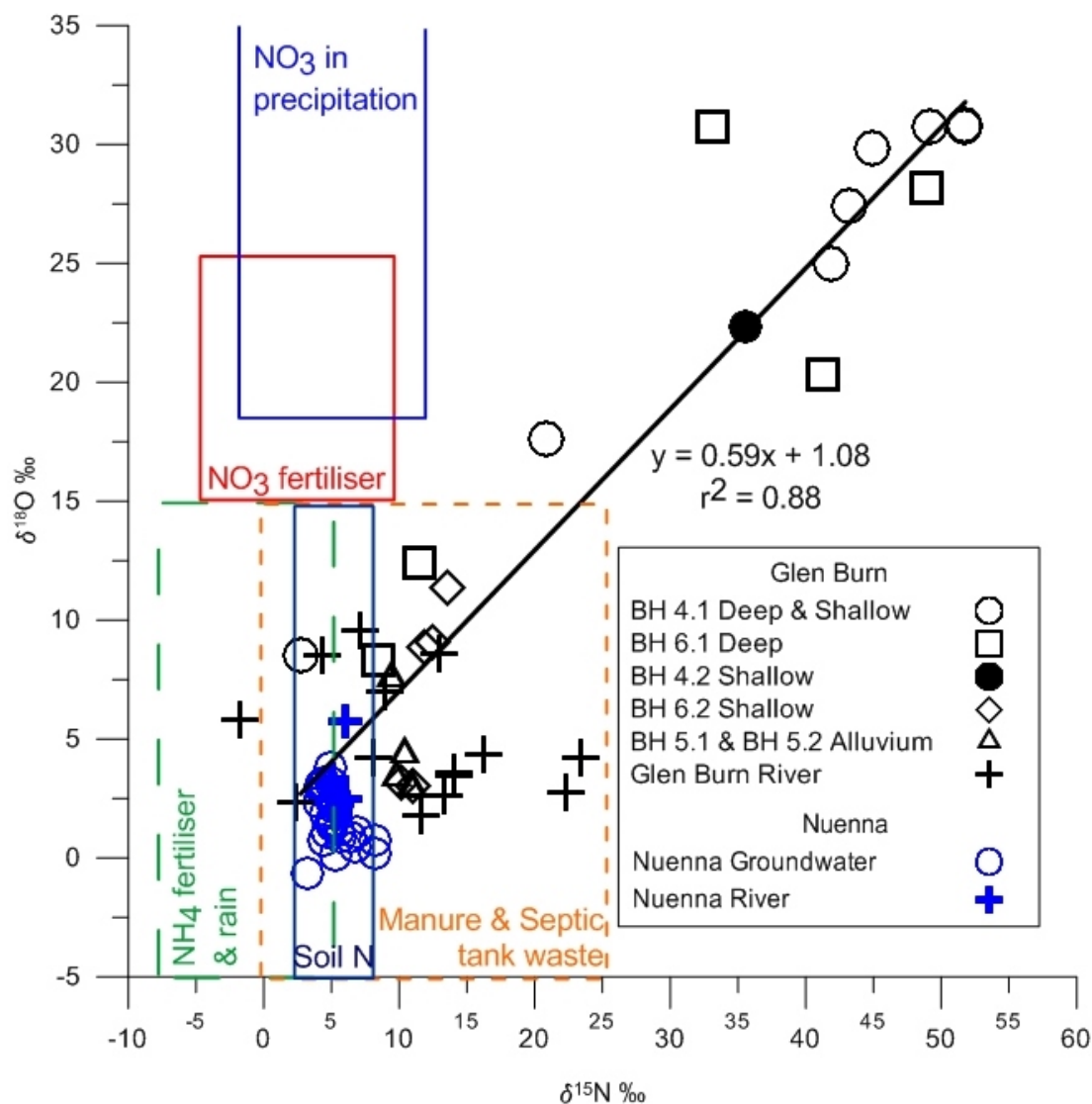
Figure 5 \delta^{15}\text{N} and \delta^{18}\text{O} in groundwater and surface water in the Glen Burn catchment. Boxes show the range of \delta^{15}\text{N} for manure and septic tank waste, \text{NH}_4 fertiliser and soil N, adapted from Kendall (1998).
