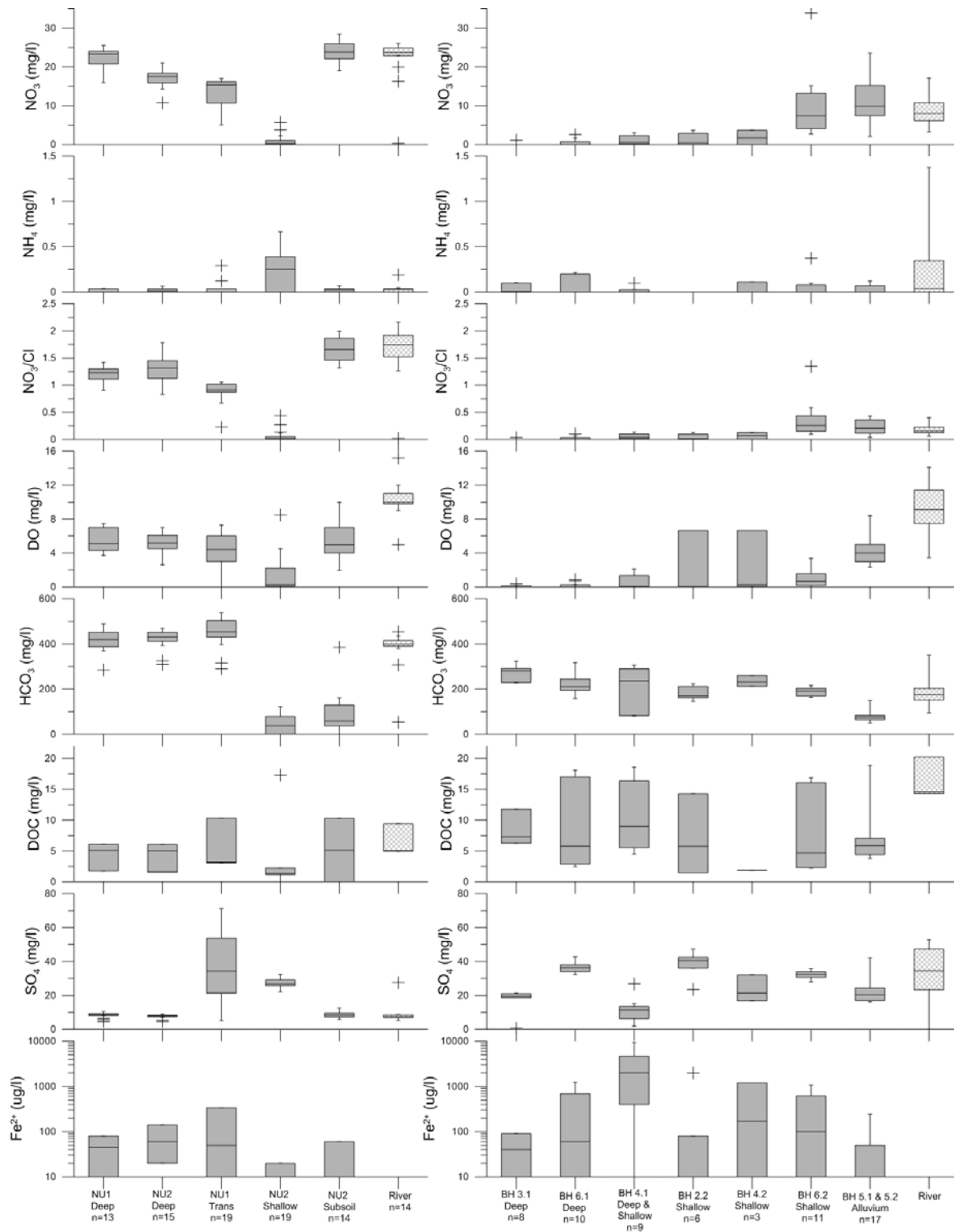
2 Figure 3 Box and whisker plots of \text{NO}_3 , \text{NH}_4 , \text{NO}_3/\text{Cl} , DO, \text{HCO}_3 , DOC, \text{SO}_4 and \text{Fe}^{2+} concentrations in 3 groundwater pathways and rivers in the Nuenna and Glen Burn catchments.
