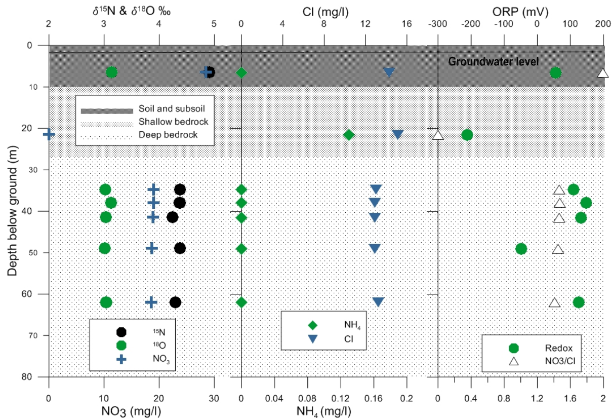
Figure 4 Variation of NO 3 , NH 4 , Cl, ORP concentrations and NO 3 isotope ( \delta^{15}\text{N} and \delta^{18}\text{O} ) values with depth in the NU2 cluster, sampled using a packer system and low flow pump.
