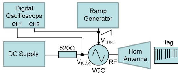
Fig. 2 Single VCO Chipless RFID reader
