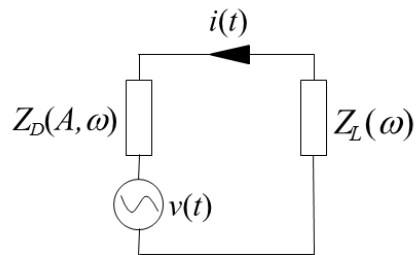
Fig. 1 Simplified oscillator equivalent circuit
