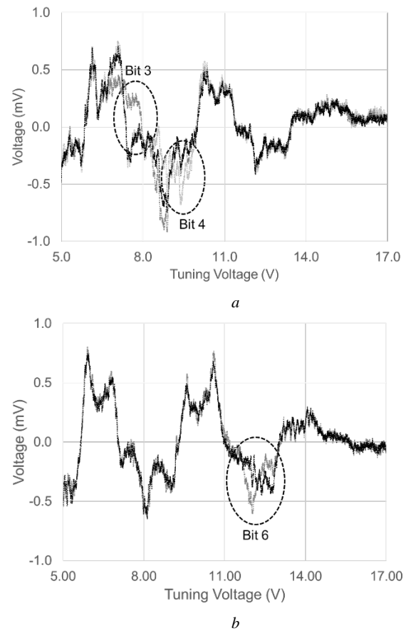
Fig. 5 Chipless RFID tag Detection using Single VCO Reader a Bits 3&4 b Bit 6
