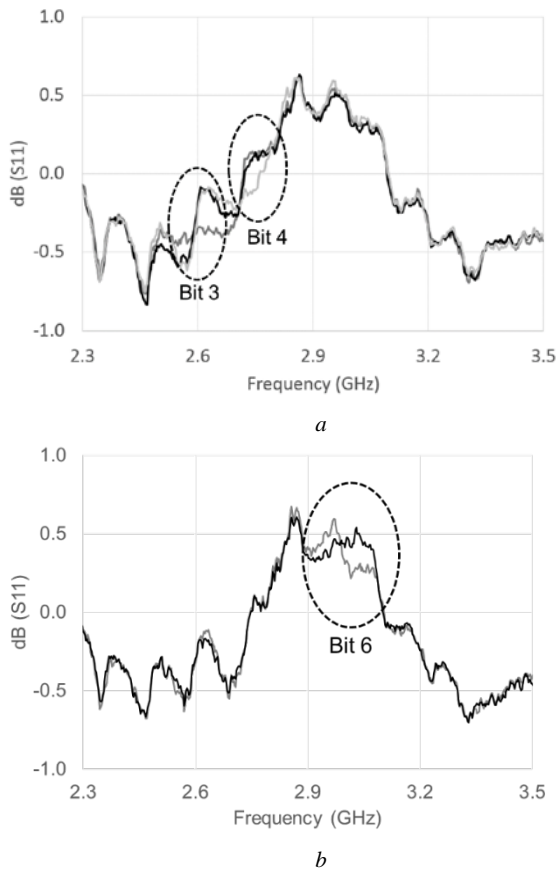
Fig. 4 Chipless RFID tag Detection using PNA a Bits 3&4 b Bit 6
