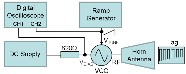
Fig. 2 Single VCO Chipless RFID reader
