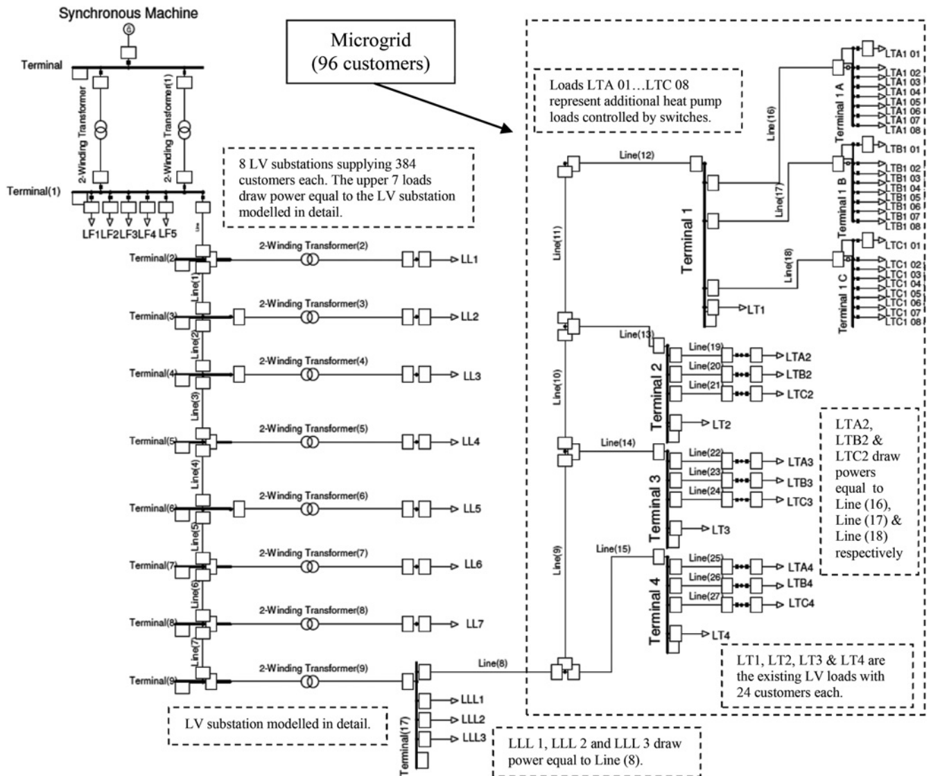
Fig. 4 Test network modelled in DiGSILENT
