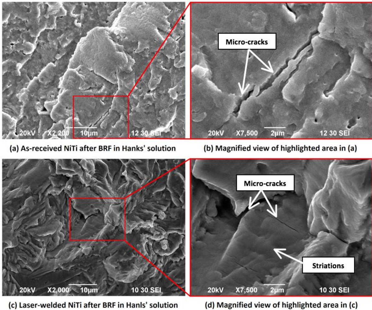
Fig. 2 – SEM fractographs for the (a-b) as-received and (c-d) laser-welded samples after testing by BRF in Hanks' solution at 37.5 °C.
