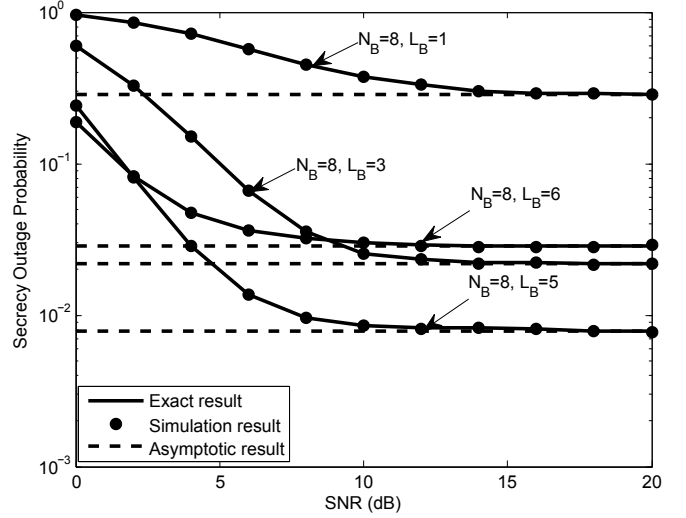
Fig. 2. Secrecy outage probability vs number of antennas for RSC/ZFB scheme, where the interference threshold Q = 10\text{dB} .
