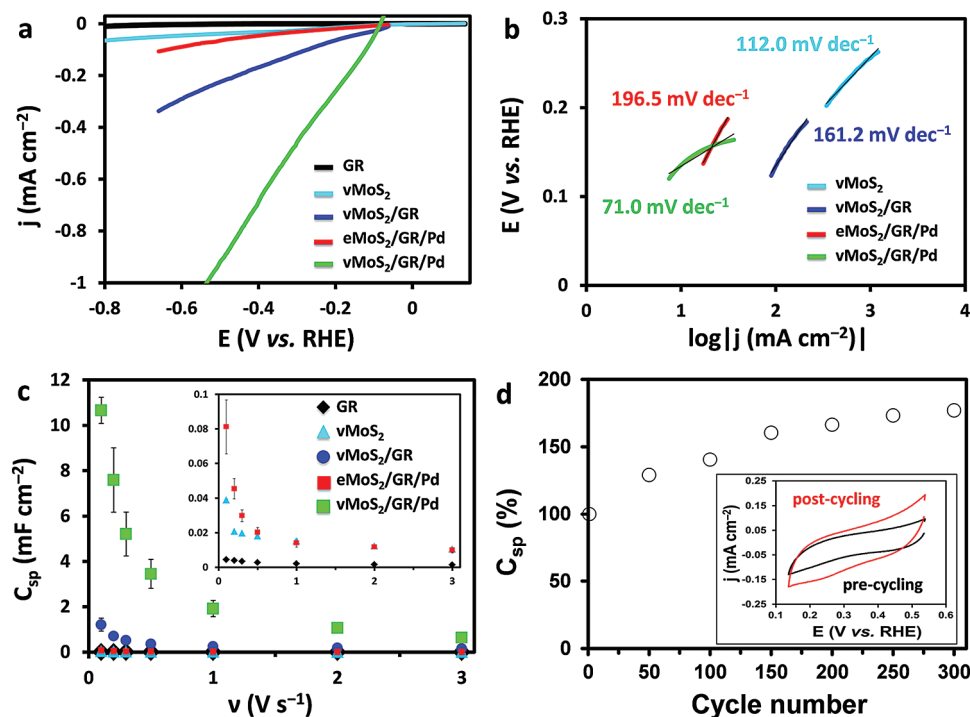
Figure 4. a) The HER polarization curves obtained on the composite materials, at 5 mV s -1 scan rate. b) Tafel slopes of HER reactions. c) Specific capacitance versus scan rate, the inset is the magnified GR, vMoS 2 , eMoS 2 /GR/Pd signals, respectively. d) Plot of the increase in specific capacitance (%) with continued cycling; the pre- and postcycling voltammograms before and after 300 cycles are shown in the inset.
