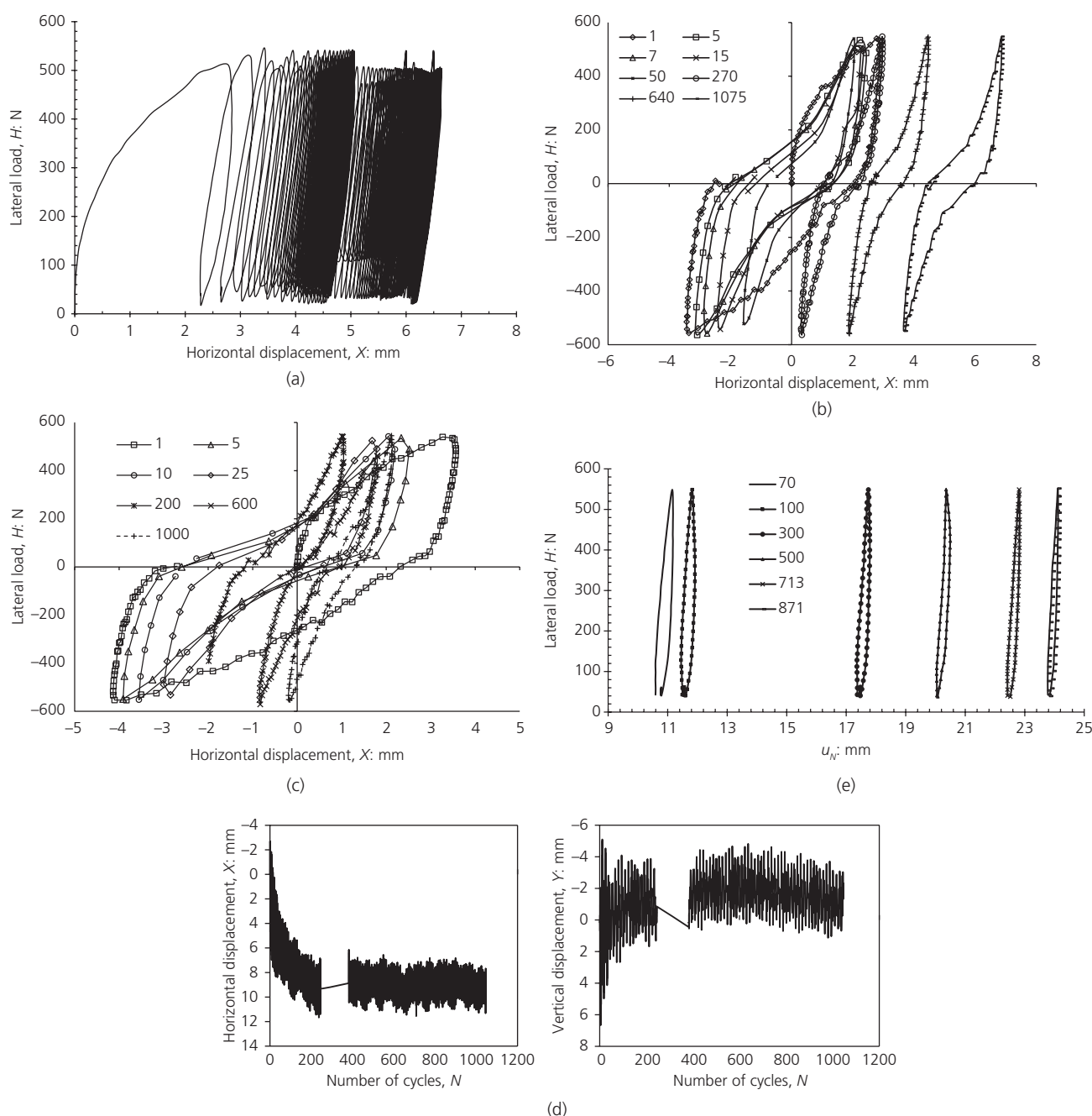
Figure 6. (a) Performance of monopile (open-ended) during lateral loading ( T_1 , U, O, \zeta=0 ). (b) Horizontal displacement and lateral load relationship at various cycles of loading for uni-directional closed-ended pile ( T_3 , U, C, \zeta=-1 ). (c) Horizontal displacement and lateral load relationship at various cycles of loading for uni-directional open-ended pile ( T_2 , U, O, \zeta=-1 ). (d) Observed pile movement along X- and Y-axis with number of cycles during multi-directional test ( T_6 , M, O, \zeta=-1 ). (e) Lateral load and u_N relationship at various cycles ( T_4 , M, O, \zeta=0 )
