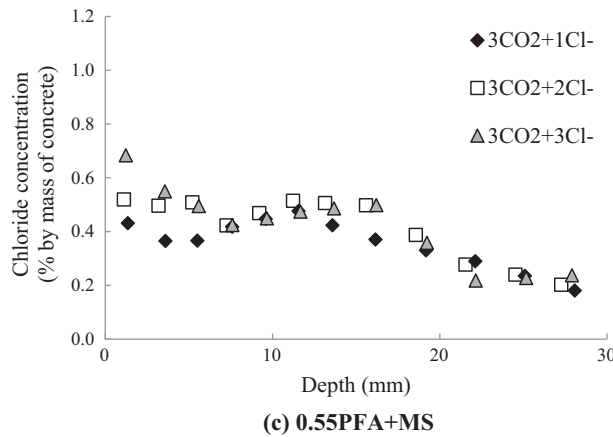
Fig. 10. Distribution of Cl - for the 3CO 2 + xCl - regime.
