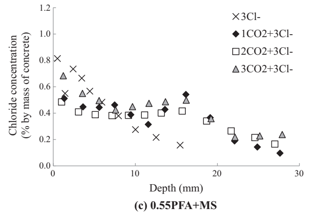
Fig. 11. Distribution of Cl - in concretes exposed to yCO 2 + 3Cl - regime.
