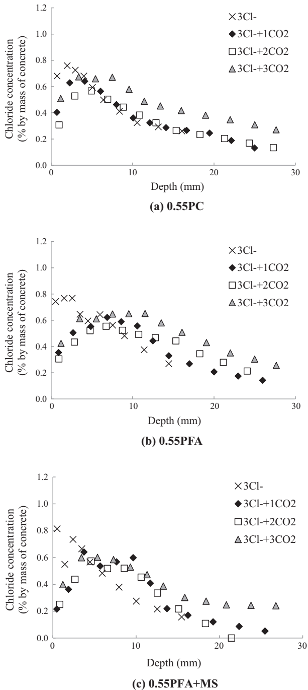
Fig. 5. Distribution of Cl - in concretes exposed to the 3Cl - + yCO 2 regime.
