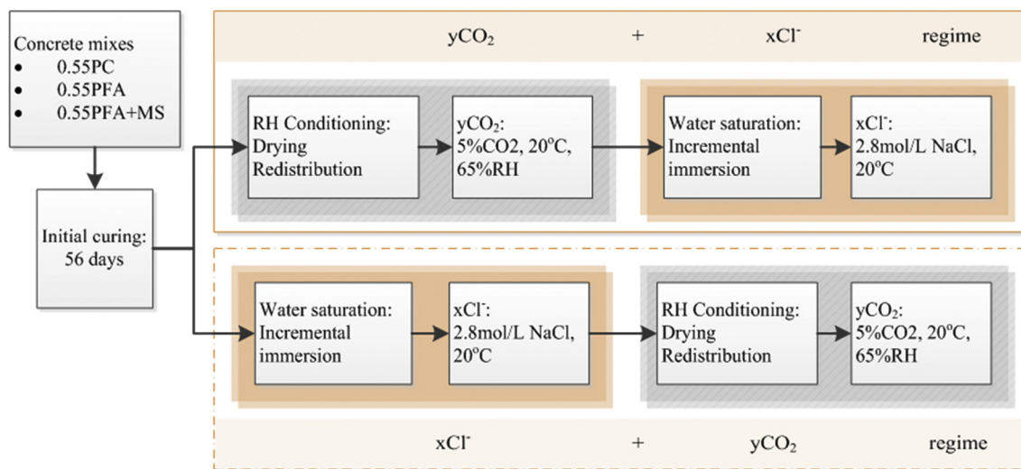
Fig. 2. Flowchart of the experimental processes.
