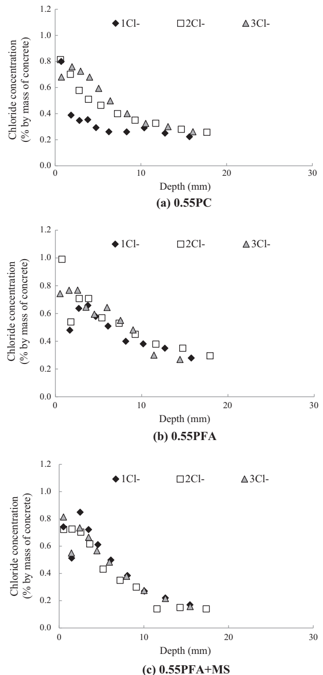
Fig. 3. Distribution of \text{Cl}^- in concretes during the x\text{Cl}^- regime.
