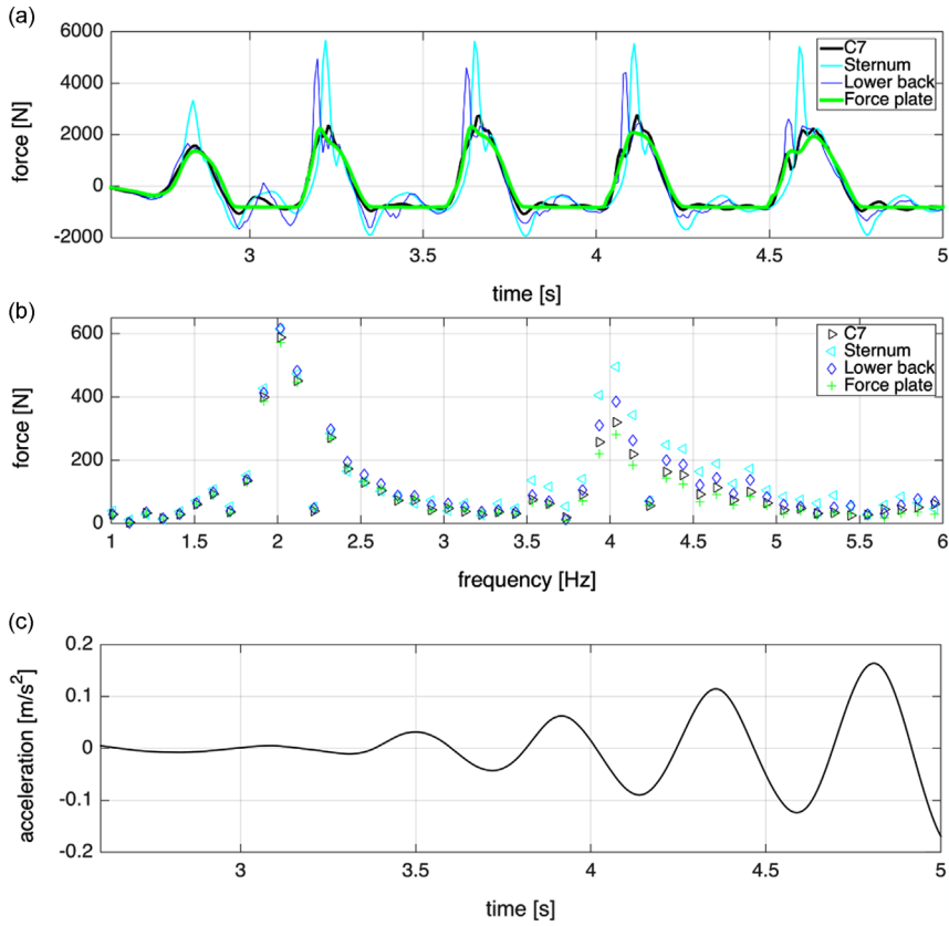
Fig. 11. Jumping forces from force plate (measured directly) and Opal™ IMUs (measured indirectly) for the second author jumping at 2 Hz between TP4 and TP21: (a) Time series, (b) Fourier line amplitudes of 10 s duration force signals of which truncated time histories are shown in (a), (c) growing deck acceleration response.
