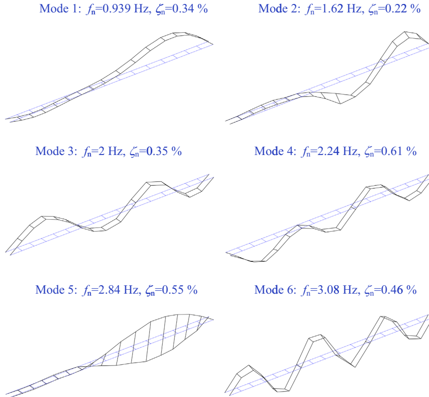
Fig. 6. Mode shapes and frequency estimates from preliminary test. Longer front span is to the right in each mode.
