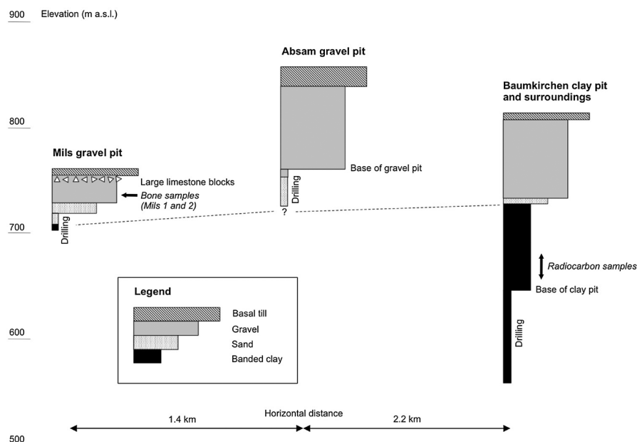
Figure 3. Simplified stratigraphic logs of the three large artificial outcrops in the Gnadewald terrace compiled from the literature (see text for references). The top of the banded clay sequence dips slightly westward (stippled line). The locations of both the original Fliri specimens from Baumkirchen and the bone fragments from the former Mils gravel pit are indicated (italics).
