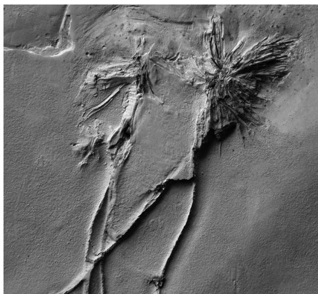
Figure 4. Example of Pinus mugo twigs with needles found in the banded clays of Baumkirchen. Width of image 17 cm. This is part of the large specimen F4 of F. Fliri, which also contained trace fossils of fish (e.g. Fliri et al. , 1971).
