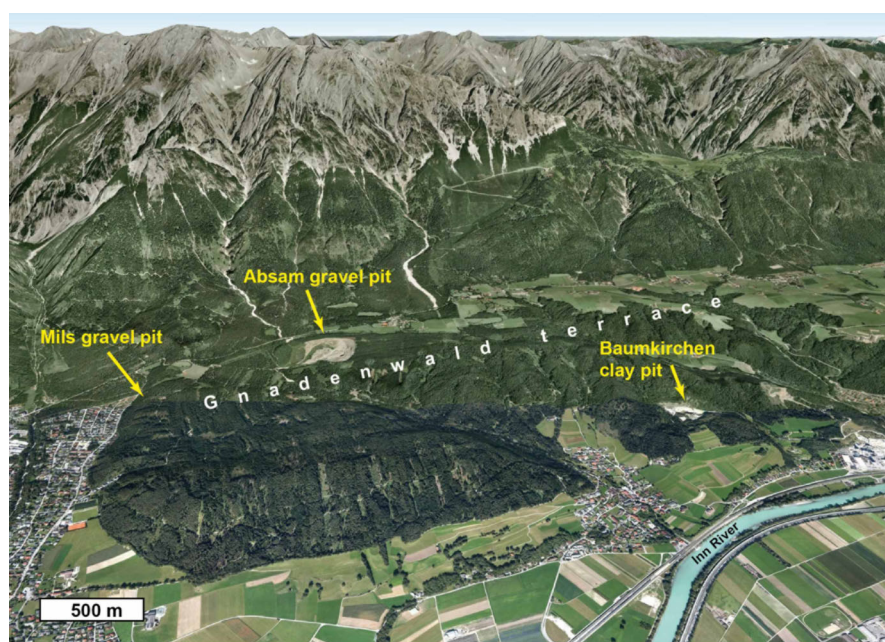
Figure 2. Oblique aerial view of the MIS 3 and 2 terrace of Gnadenwald located some 250 m above the Inn River and the adjacent Karwendel Mountains to the north (Google Earth Pro image). The Baumkirchen clay pit is located near the southern (erosional) rim of the terrace, whereas the Absam gravel pit is situated on the plateau. The former Mils gravel pit opened on the western side of the terrace and was later back-filled and re-vegetated. This figure is available in colour online at wileyonlinelibrary.com .
