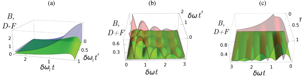
FIG. 2. (Color online) Effects of system-environment correlations described through the function B(t', t, \rho^{1,2}) given in Eq. (26) corresponding to the example discussed in Sec. III A for a frequency distribution as in Eq. (28). (a) We have taken \omega_1^0/\delta\omega_1 = \omega_2^0/\delta\omega_1 , \delta\omega_2/\delta\omega_1 = 10 , and r = 1 . In both (b) and (c) we have taken \delta\omega_{1,2} \equiv \delta\omega , \omega_1^0/\delta\omega = 1 , and \omega_2^0/\delta\omega = 9 with r = 1 ( t'\delta\omega = 0.3 ) in (b) [(c)]. Semitransparent surfaces represent D(t, \rho^{1,2}) - F(t', t, \rho^{1,2}) (a) and D(t, \rho^{1,2}) + F(t', t, \rho^{1,2}) [(b) and (c)].
