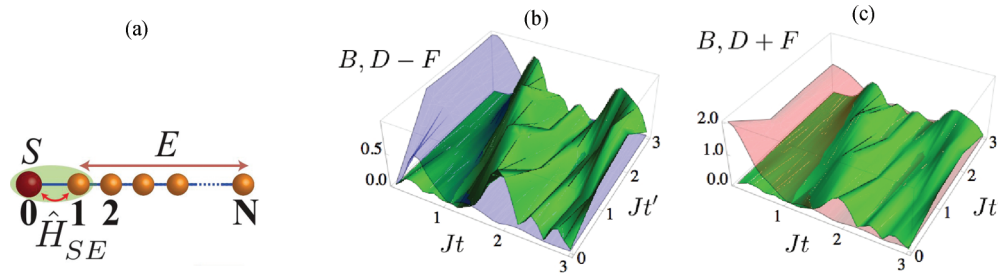
FIG. 3. (Color online) (a) We consider a quantum spin chain of N + 1 particles partitioned into a two-level-system spin embodied by particle 0 and a finite-size environment (provided by the rest of the chain). The dynamics experienced by spin 0 can be changed from Markovian to strongly non-Markovian by adjusting the parameters entering the system-environment coupling model \hat{H}_{SE} and the interenvironment one \hat{H}_E . Details of the form of such Hamiltonians are given in the body of the paper. (b) [(c)] Comparison between the function B(t', t, \rho^{1,2}) (full-color surface) and the threshold for Markovianity (non-Markovianity) D(t, \rho^{1,2}) - F(t', t, \rho^{1,2}) [ D(t, \rho^{1,2}) + F(t', t, \rho^{1,2}) ]. (semitransparent curves). We have used N = 8 with J_0/J = 1 and B/J = 10^{-2} .
