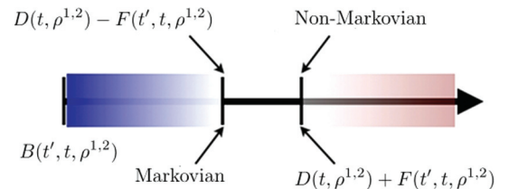
FIG. 1. (Color online) The horizontal axis represents the possible values of B defined in Eq. (5) at fixed times t and t' and initial reduced states \rho_S^1(0) and \rho_S^2(0) , while the two marks represent the thresholds given by D(t, \rho^{1,2}) - F(t', t, \rho^{1,2}) (blue region, lower mark) and D(t, \rho^{1,2}) + F(t', t, \rho^{1,2}) (red region, upper mark), with D(t, \rho^{1,2}) and F(t', t, \rho^{1,2}) defined in Eqs. (7) and (4), respectively. If B(t', t, \rho^{1,2}) lies above the upper threshold for some t, t', \rho_S^{1,2}(0) , the dynamics is non-Markovian, while if it takes values below the lower threshold for all the t, t', \rho_S^{1,2}(0) , the dynamics is Markovian. Values of B(t', t, \rho^{1,2}) between the two thresholds are compatible with both Markovian and non-Markovian dynamics.
