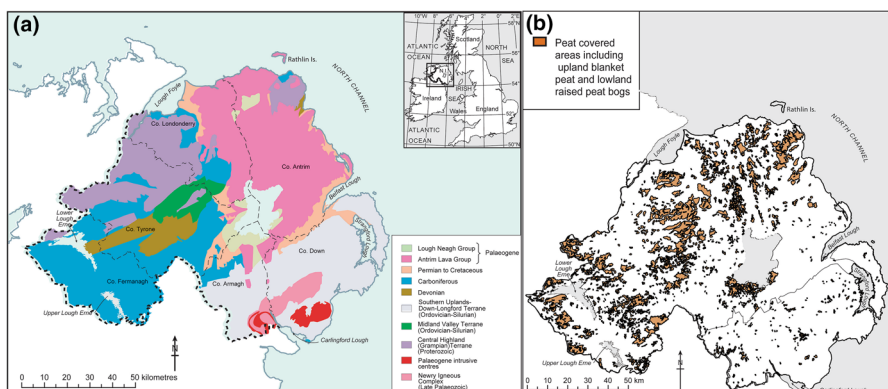
Fig. 1 a Simplified geology of Northern Ireland (after Mitchell 2004); b map showing post-glacial peat-covered areas
