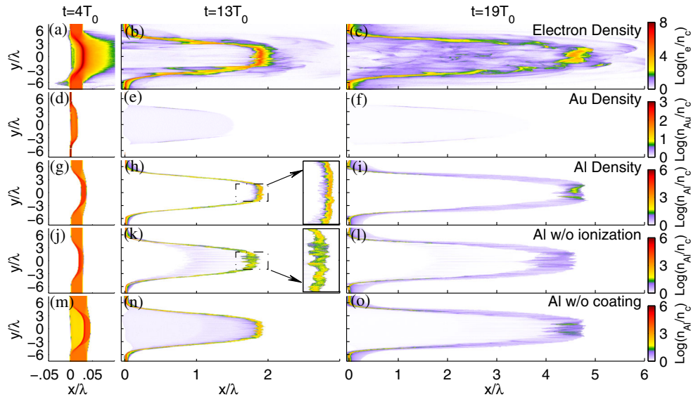
FIG. 3. Electron density \ln(n_e/n_c) (a)–(c), Au ion density \ln(n_{\text{Au}}/n_c) (d)–(f), Al ion density \ln(n_{\text{Al}}/n_c) (g)–(i) at t = 4, 13 and 19T_0 in the acceleration of an Al foil by laser at I_0 = 10^{22} \text{ W/cm}^2 , where a 2 nm Au coating is used. The Al ion density for the cases without ionization effect (j)–(l) and without the Au coating (m)–(o) are also plotted. Insets show zoomed density maps in the dotted-dashed boxes, which indicates the seriousness of the RT instability.
