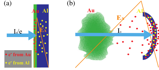
FIG. 2. Schematic of stable heavy ion RPA via successive electron replenishment from ionization of a high- Z coating. (a) Laser fields ionize Au and Al, expelling Au electrons into Al. (b) The successive ionized electrons from the Au coating catch up and comove with the accelerating Al foil, keeping a negative gradient electric field for stable RPA.
