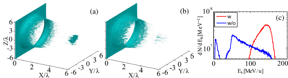
FIG. 5. 3D PIC simulation results: the Al^{13+} density isosurface for n = 3n_c with (a) and without (b) the ionization effect at t = 20T_0 . (c) The corresponding energy spectra of Al^{13+} within r < 2 \mu\text{m} with (red curve) and without (blue curve) the ionization effect.
