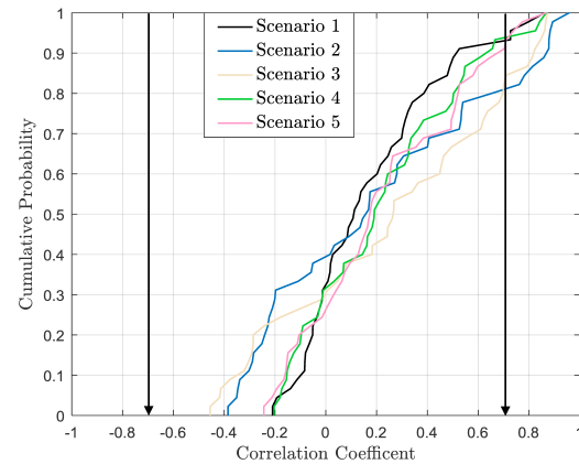
Fig. 4. CDFs of the calculated cross-correlation coefficients for all of the considered scenarios.
