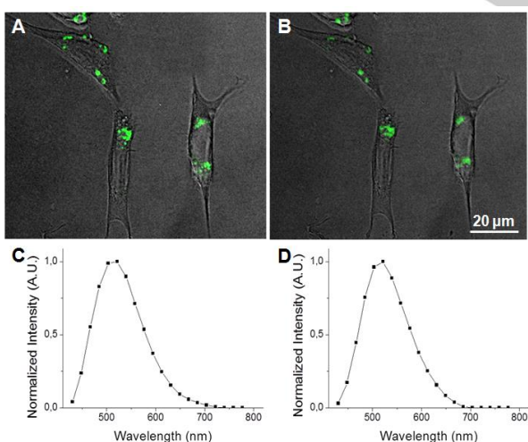
Figure 6. Confocal microscope image of POS 1 cells after 8 h of incubation with dye 3 ( 300\ \text{nm} in the media): merge of transmission image (in grey) and fluorescence image (green) showing the internalisation of the dye within the cells: (A) one-photon excitation ( \lambda_{\text{ex}} = 405\ \text{nm} ; \lambda_{\text{em}} = 500\text{--}600\ \text{nm} ) and (B) two-photon excitation ( \lambda_{\text{ex}} = 800\ \text{nm} ; \lambda_{\text{em}} = 500\text{--}600\ \text{nm} ); (C) emission spectrum upon one-photon excitation ( \lambda_{\text{ex}} = 405\ \text{nm} ; 20\ \text{nm} step) of the dye within the cell; (D) emission spectrum upon two-photon excitation ( \lambda_{\text{ex}} = 800\ \text{nm} ; 20\ \text{nm} step) of the dye within the cell.
