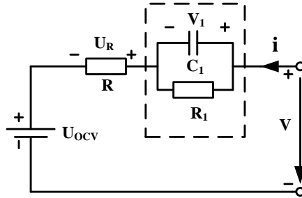
Fig. 1. Battery Thevenin model.
