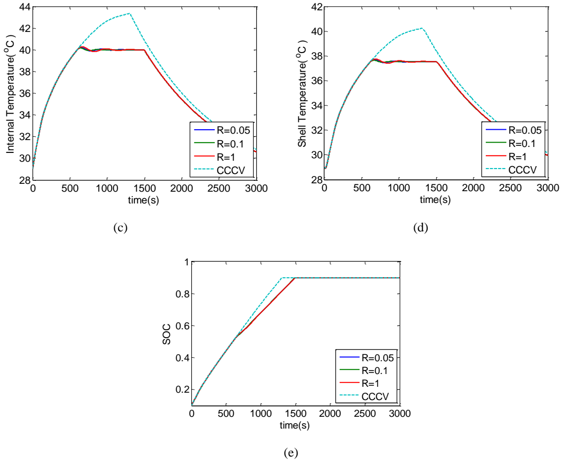
Fig. 5. Effect of control penalty weight, R ( N_c = 2, N_p = 60 )
