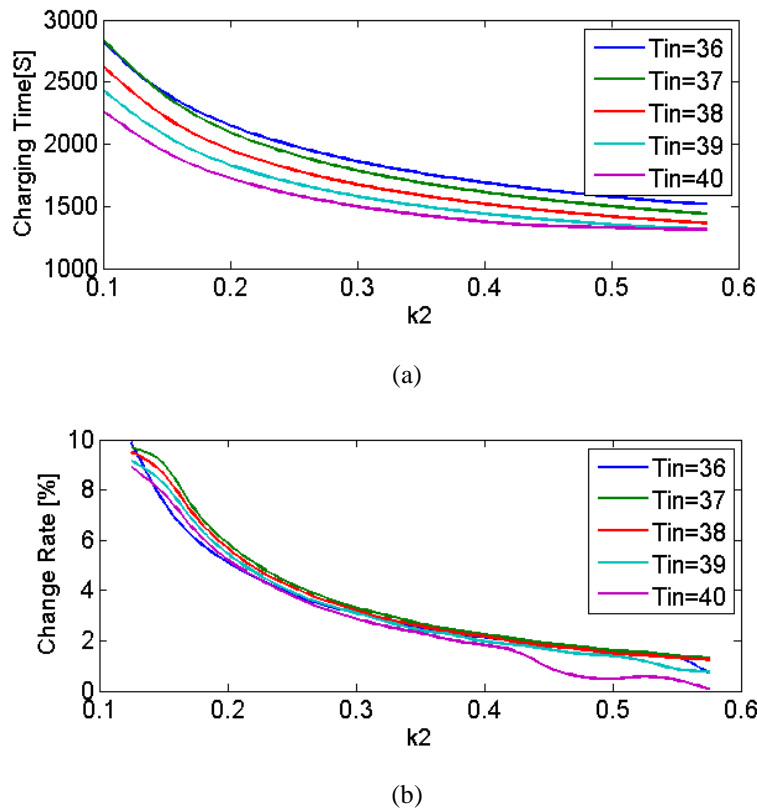
Fig. 7. Relations of charging time with dissipation rates.(a) Charging time (b) Change rate of charging time
