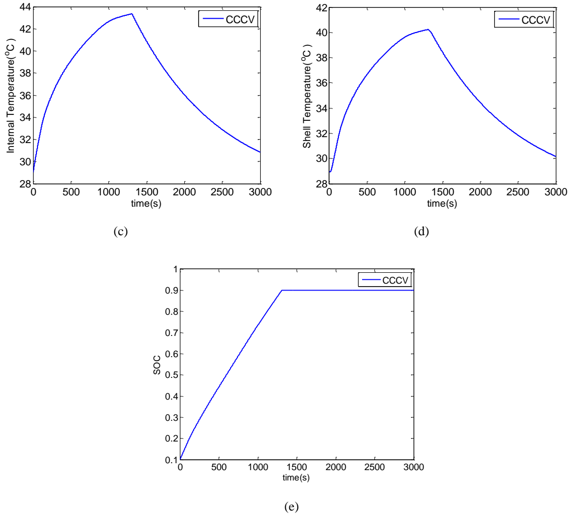
Fig. 3. Battery cell charging profile with CCCV method ((a) charge current, (b) terminal voltage (c) internal temperature, (d) shell temperature, (e) SOC)
