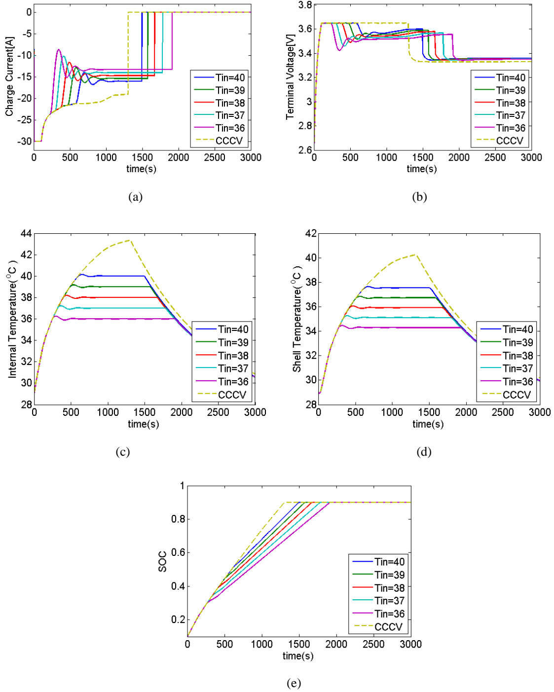
Fig. 8. Effect of different internal temperatures ( N_c = 2, N_p = 60, R = 0.05 )
