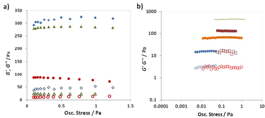
Fig. 7. Stress dependence of emulsion storage ( G' , solid symbols) and loss modulus ( G'' , empty symbols) in the near viscoelastic re-gion: a) comparison among different HFBI concentrations: 0.25 ( \bullet ), 0.5 ( \blacktriangle ), and 1 mg/mL ( \blacklozenge ); b) comparison among different surfac-tants: Brij 1 mg/mL ( \blacklozenge ), SDS 2 mg/mL ( \bullet ), SDS 3 mg/mL ( \blacksquare ), and HFBI 2.5 mg/mL ( \circ ).
