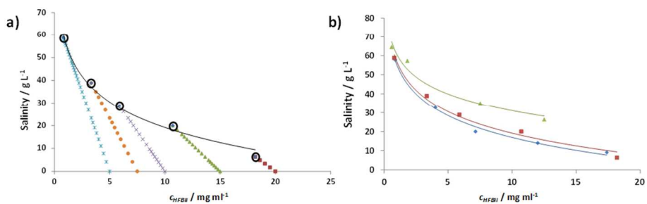
Fig. 1. a) Titration curves, showing salinity values versus different HFBII concentrations: 5 ( \nabla ), 7.5 ( \bullet ), 10 ( \times ), 15 ( \blacktriangle ), and 20 mg/mL ( \blacksquare ). Flocculation points for each series are marked with a black circle. b) Flocculation points obtained at different temperatures, varying HFBII concentration: 20 °C ( \blacksquare ), 40 °C ( \blacklozenge ), and 70 °C ( \blacktriangle ).
