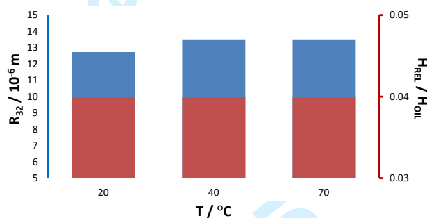
Fig. 5. Effect of thermal treatment at different temperatures on mean volume-surface radius ( R_{32} , blue) and relative volume of oil released from emulsions after centrifugation ( H_{REL}/H_{OIL} , red).
