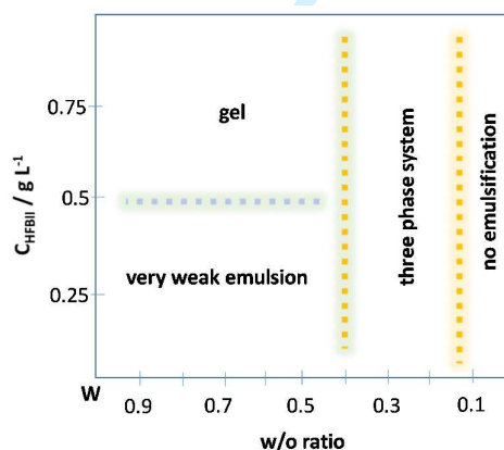
Fig. 8. Phase behaviour diagram of the studied emulsions, as a function of protein concentration ( C_{\text{HFB}} ) and w/o ratio.
