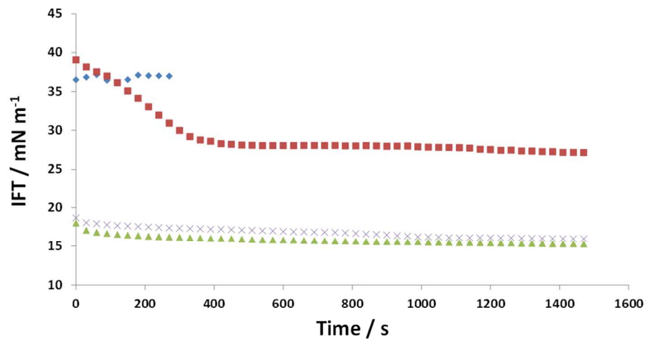
Fig. 2. Interfacial tension trends over time for SSW solutions of HFBI at different protein concentrations: 0 (♦), 0.01 (■), 0.1 (▲), and 1 mg/mL (×).
