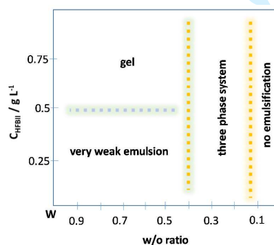
Fig. 8. Phase behaviour diagram of the studied emulsions, as a function of protein concentration ( C_{\text{HFBII}} ) and w/o ratio.
