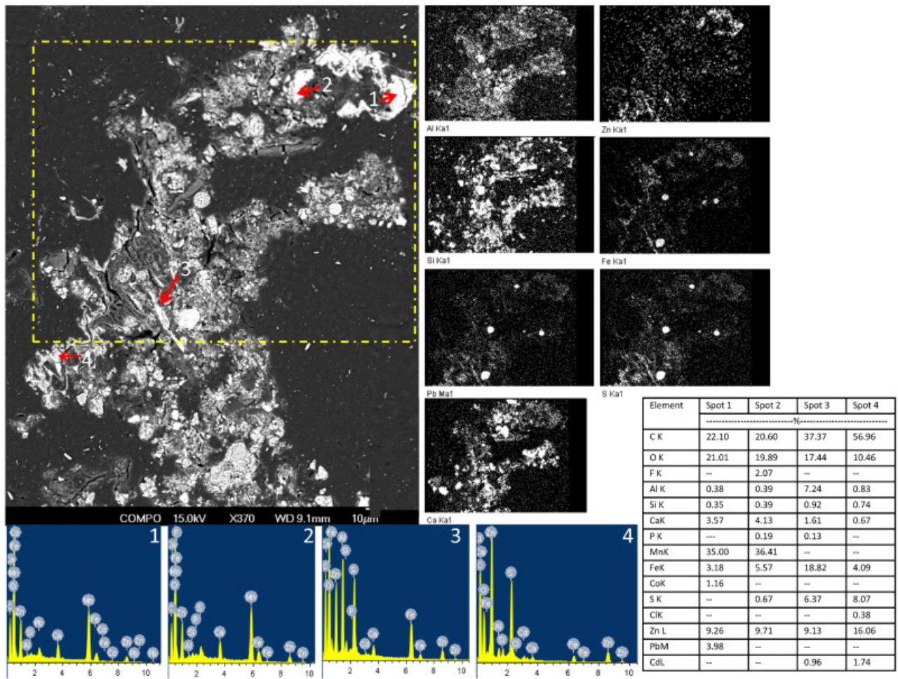
Fig. 7 Photomicrograph, WDS elemental maps and analysis and SEM-EDS analysis of a fragment of peat encrusted with metals including Zn, Cd, and Pb.
