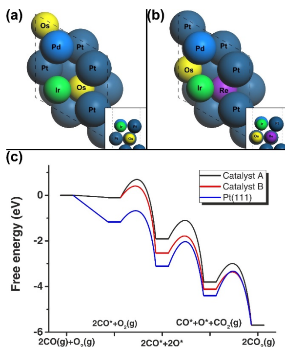
Figure 3. Top views and side views (inset) of (a) catalyst A and (b) catalyst B, and (c) the energy profiles of CO oxidation on catalyst A (black), catalyst B (red) and Pt(111) (blue). The free energies in (c) were obtained using DFT calculations.
