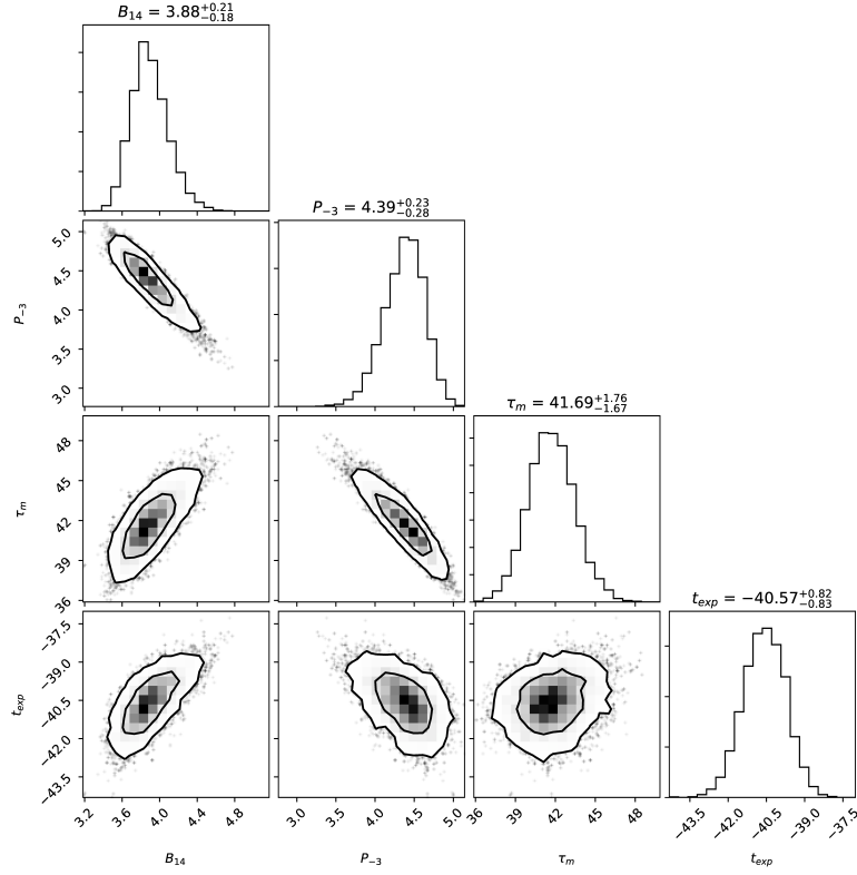
Figure B22. Confidence levels of the best-fit parameters for the magnetar model of PTF 10hgi.
