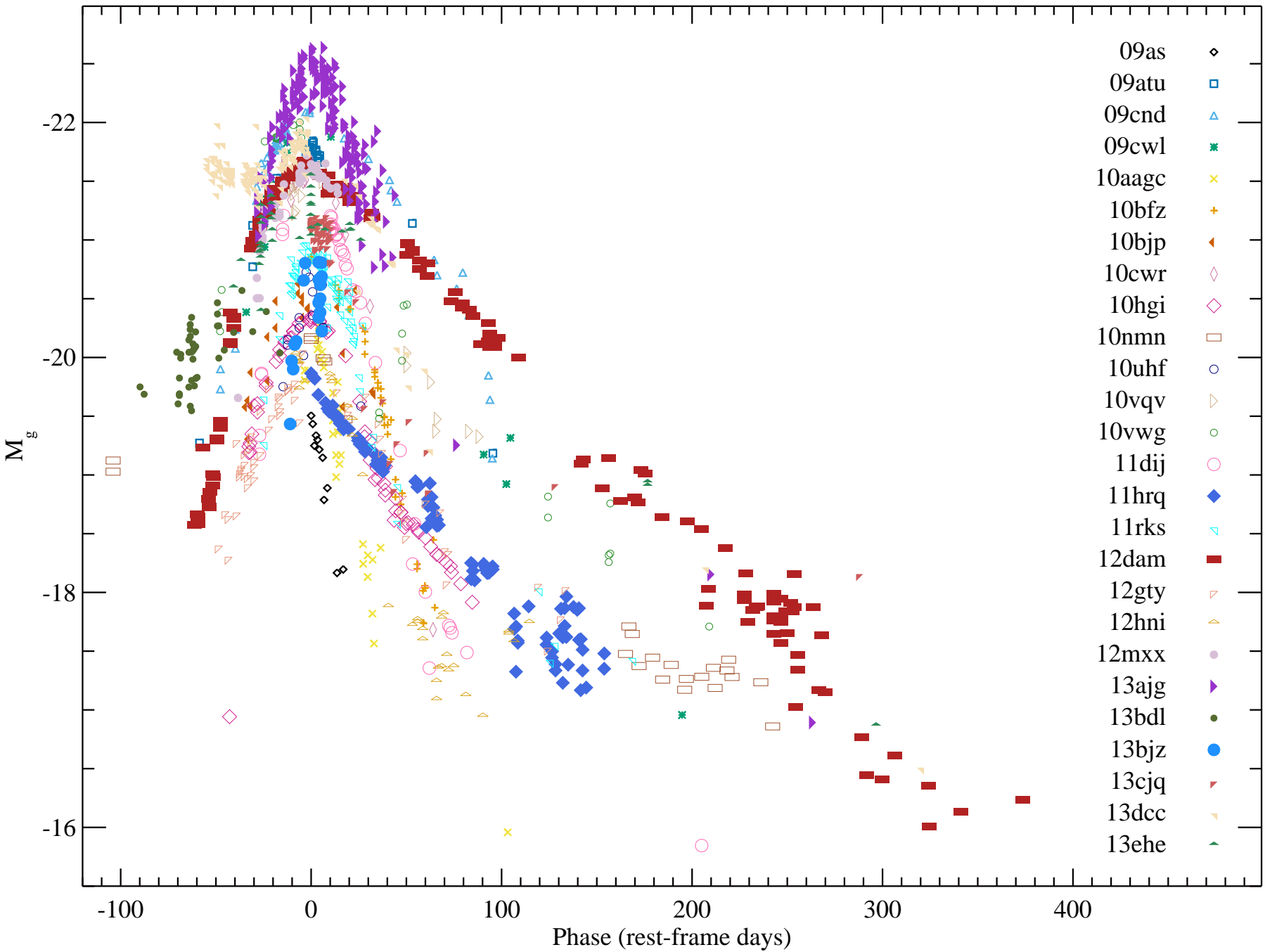
Figure 1. The rest-frame M_g light curves of the 26 H-poor SLSNe in our sample. The error bars are omitted here for readability, but are shown in Figs. B1 to B5.
