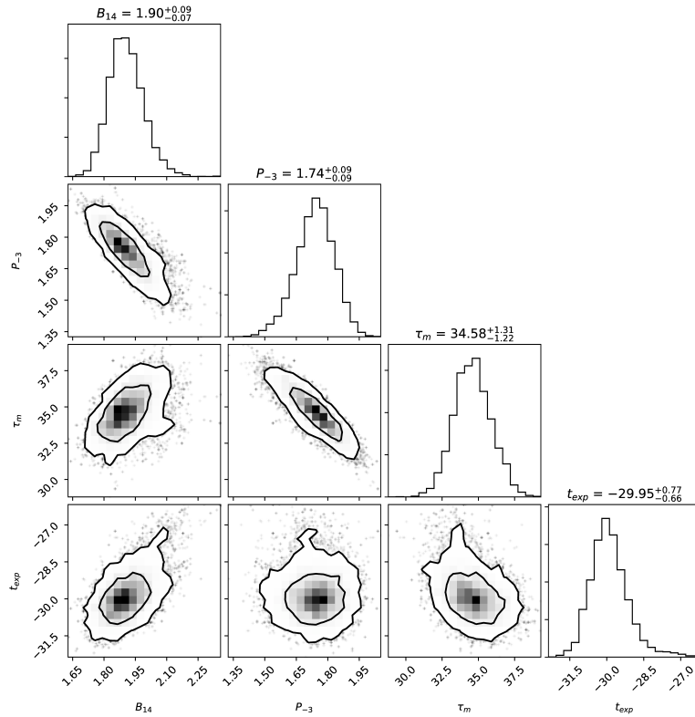
Figure B31. Confidence levels of the best-fit parameters for the magnetar model of PTF 13ajg.
