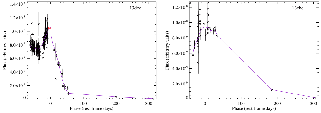
Figure B10. Continuation of Fig. B6.
