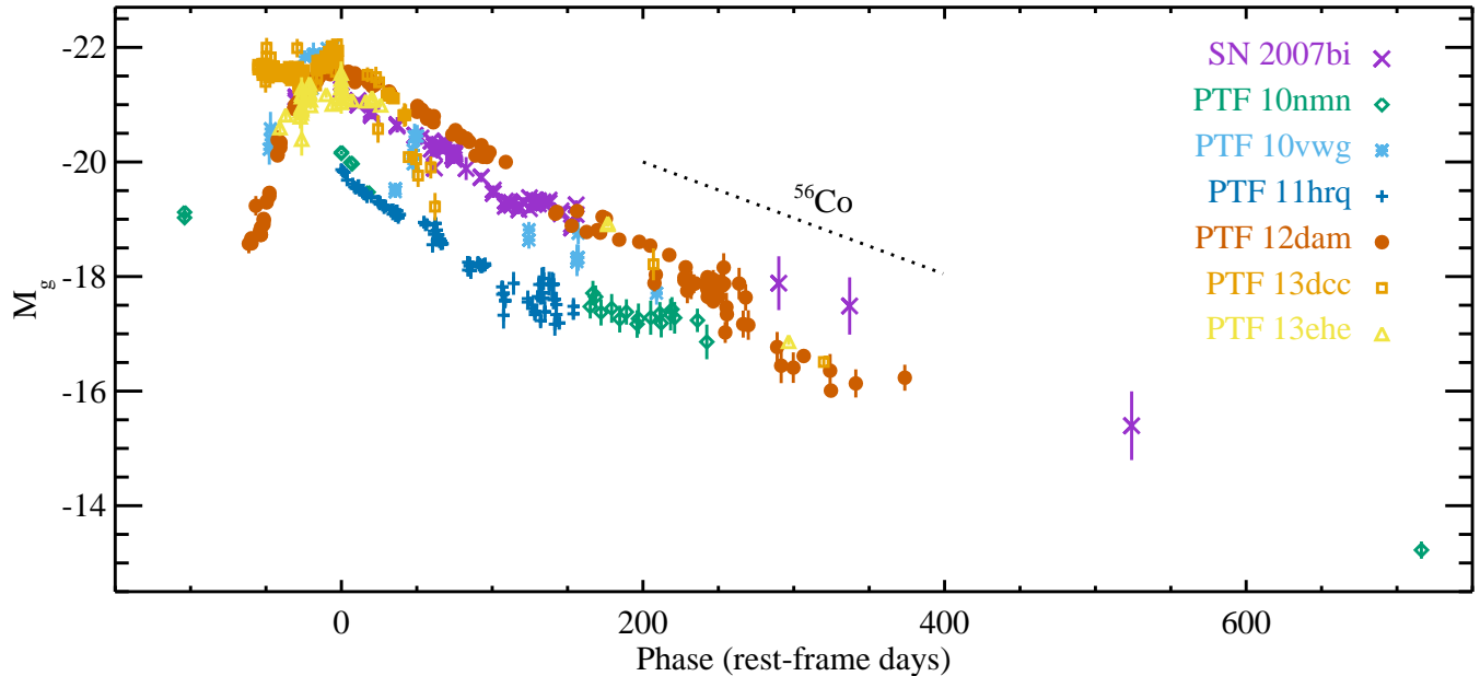
Figure 9. The rest-frame M_g light-curves of the SLSNe originally classified as SLSN of the R type
