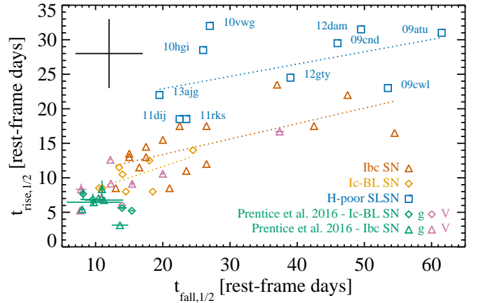
Figure 7. Times to rise and decay by half-flux. The dotted curves show linear fit to the data in our sample. The black cross shows the typical uncertainties, see text.
