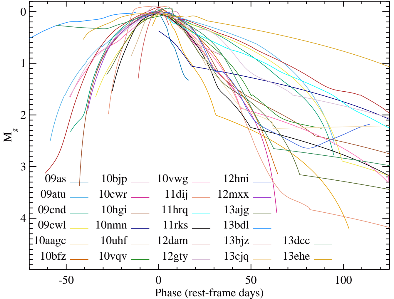
Figure 5. The rest-frame g -band smoothed light-curves of the SLSNe in our sample, normalized at peak. PTF 10nmn is normalized with respect to the peak magnitude, which is taken from Yaron et al. (in prep.) and is not presented in this paper. The peak magnitudes are derived with a second order polynomial fit to the data (Figs. B1 to B5) and reported in Table A1.
