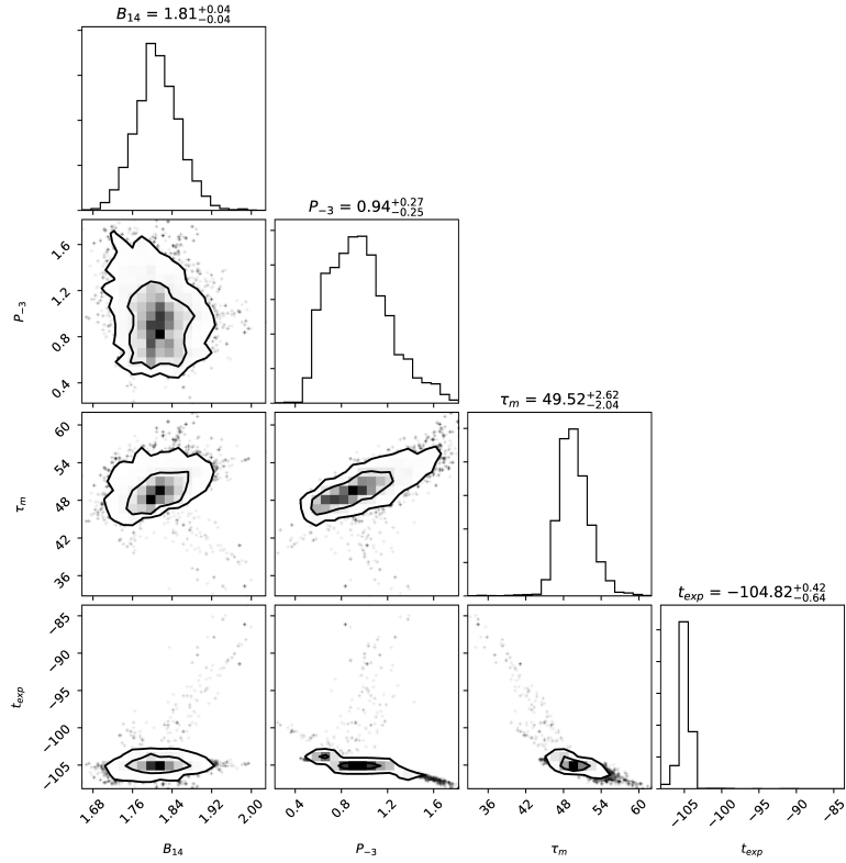
Figure B23. Confidence levels of the best-fit parameters for the magnetar model of PTF 10mn.
