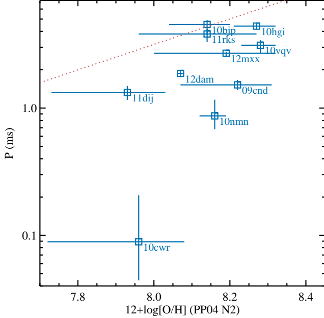
Figure 15. Magnetar spin and host-galaxy metallicity. The red dotted line shows the spin-metallicity correlation found by Chen et al. (2016) . a Best-fit parameters < 10^{-4} ms.
