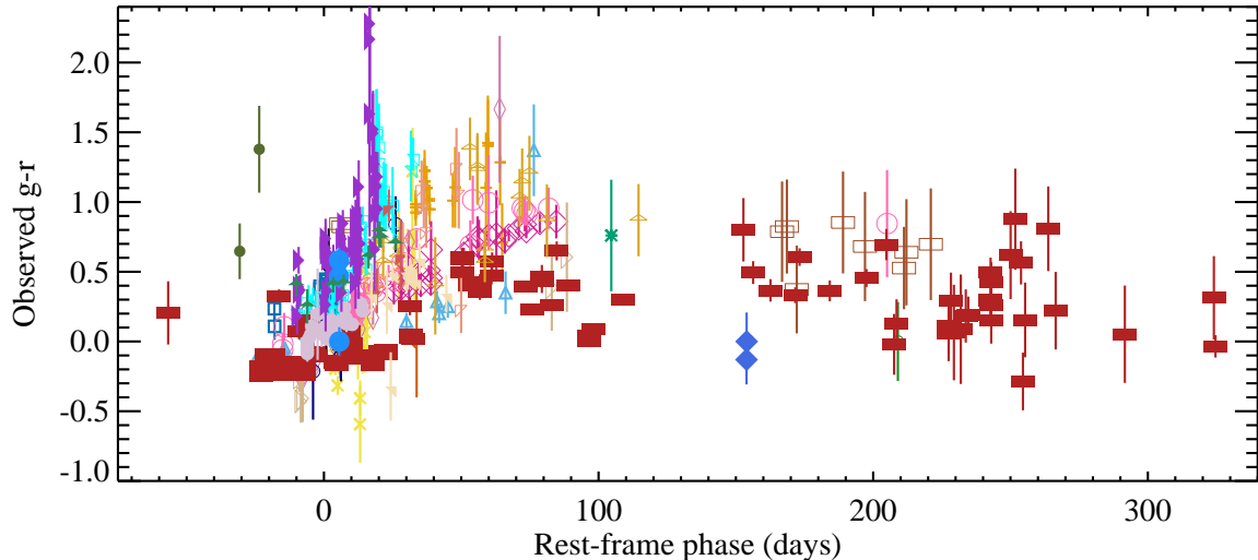
Figure 8. The observed g - r color of the SLSNe in our sample. The symbols and color are as in Fig. 1.
