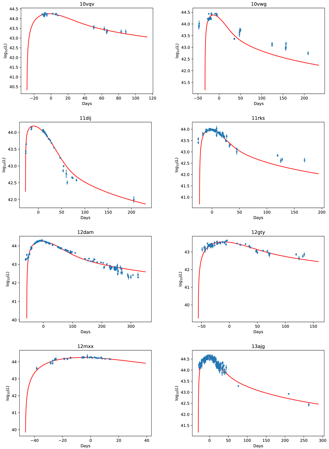
Figure B17. Continuation of Fig. B16.
