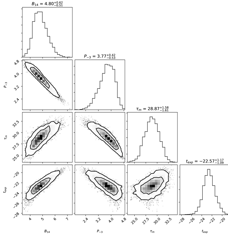
Figure B27. Confidence levels of the best-fit parameters for the magnetar model of PTF 11rks.
