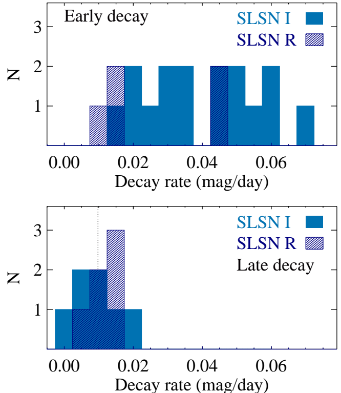
Figure 4. The post-peak decay slope distribution at early times (typically below 60 days, top panel) and at late times (typically beyond 60 days, bottom panel). At late times all observed SLSNe cluster around the ^{56}\text{Co} to ^{56}\text{Fe} decay rate of 0.0098 mag/day (dotted vertical line).
