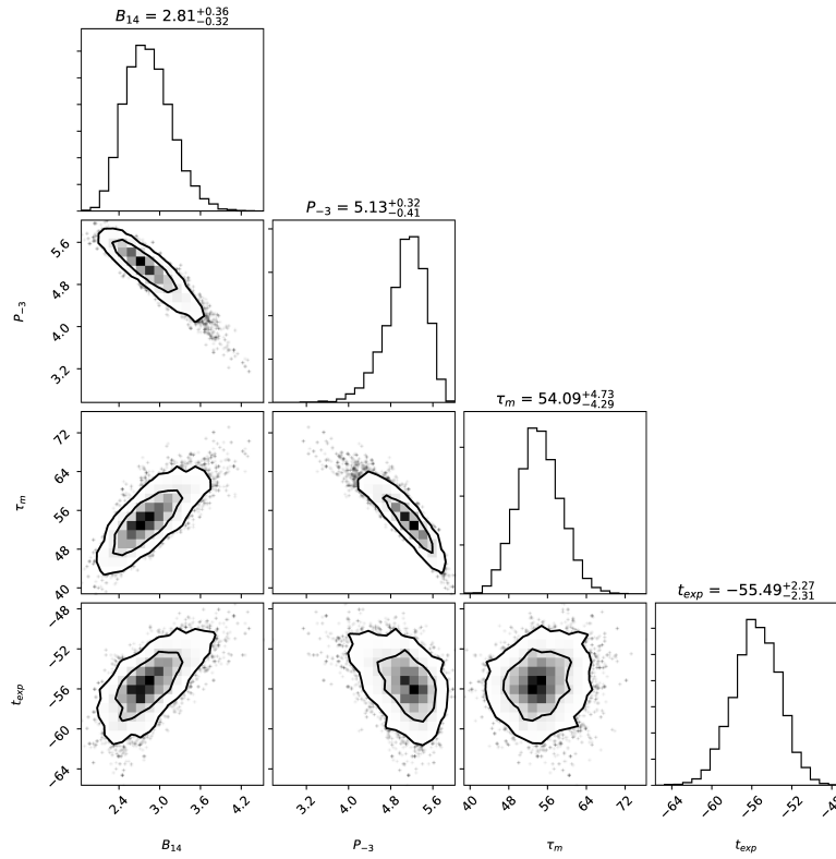
Figure B29. Confidence levels of the best-fit parameters for the magnetar model of PTF 12gty.
