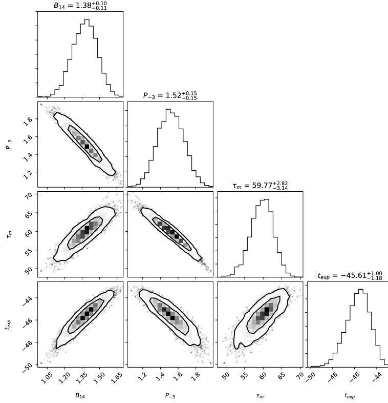
Figure B18. Confidence levels of the best-fit parameters for the magnetar model of PTF 09cnd.
