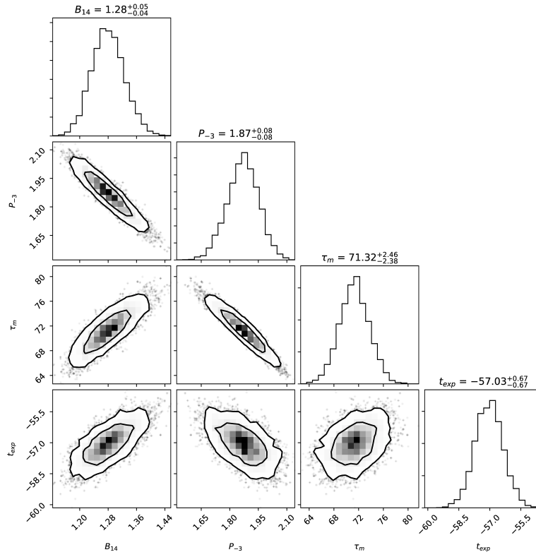
Figure B28. Confidence levels of the best-fit parameters for the magnetar model of PTF 12dam.
