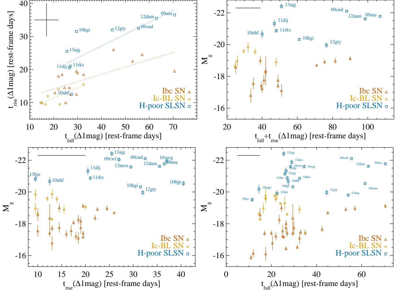
Figure 6. Times to rise and decay by 1 magnitude to and from the peak, and peak magnitudes (rest-frame g ). The dotted curves show linear fits to the data in our sample. The black cross and bars show the typical uncertainties, see text.
