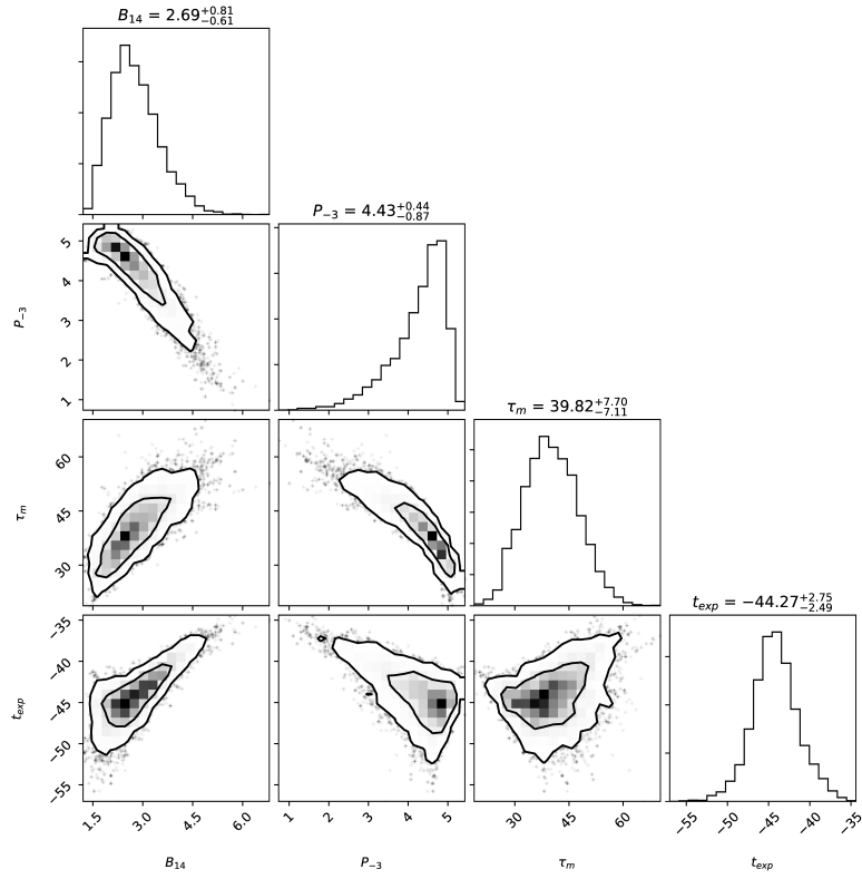
Figure B20. Confidence levels of the best-fit parameters for the magnetar model of PTF 10bjp.
