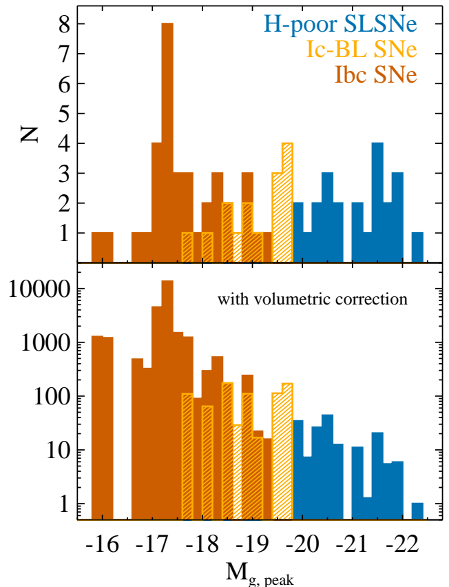
Figure 3. The peak-magnitude distribution of PTF SNe of the labelled types, for rest-frame g absolute magnitudes. The bottom panel shows the peak-magnitude distribution after volumetric correction (i.e. corrected for Malmquist bias).
