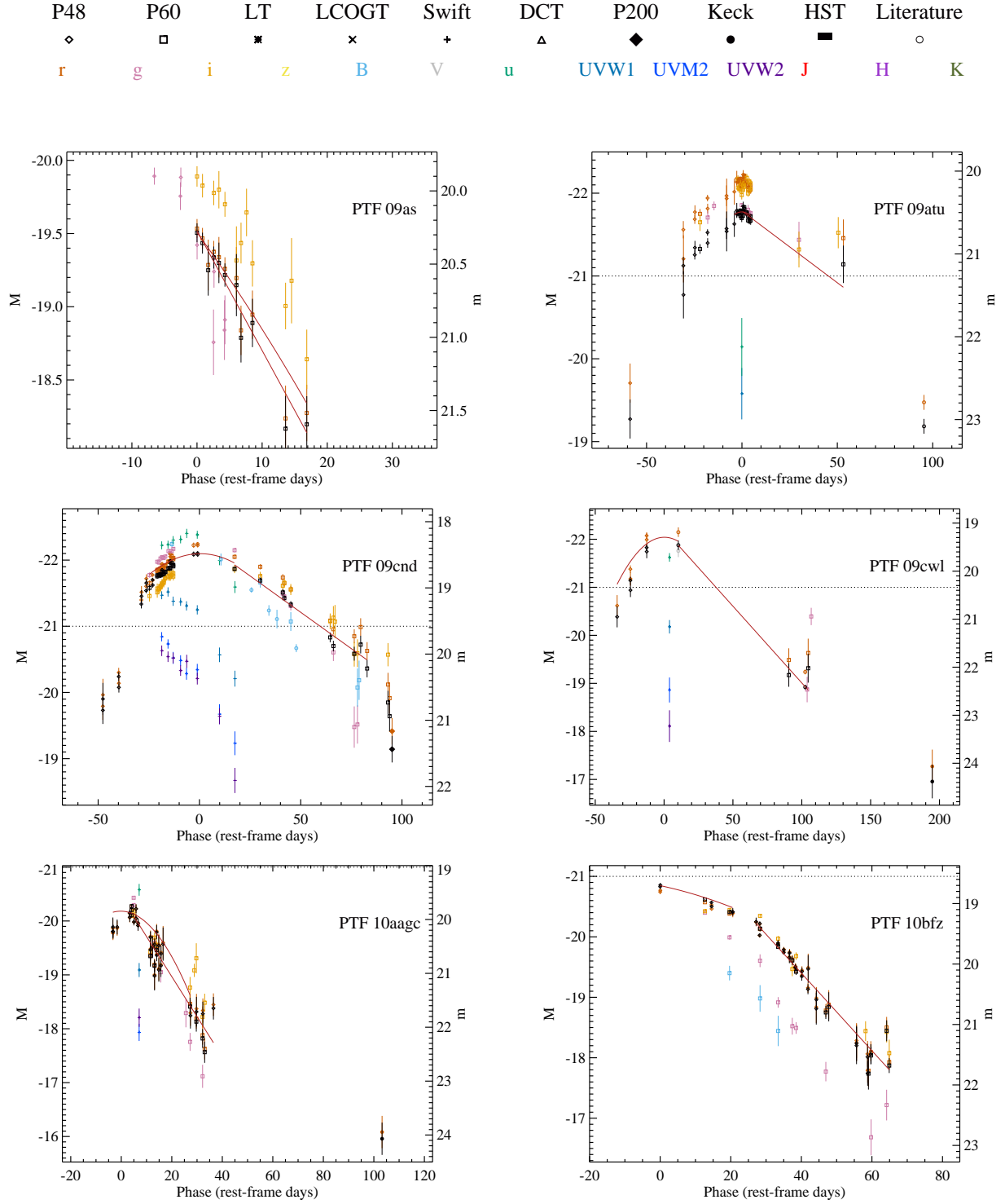
Figure B1. The light curves of (i)PTF SLSNe-I in our sample for individual observed filters, and rest-frame M_g (black). Both apparent and absolute magnitudes are corrected for Galactic foreground dust extinction (see Sect. 3.11). The solid lines show the second-order polynomial fit around peak (Sect. 4.1) and the post-peak early- and late-time decay linear fits to the data (Sect. 4.2). The horizontal dotted line marks the M = -21 mag "historical" threshold for SLSNe, for comparison.
