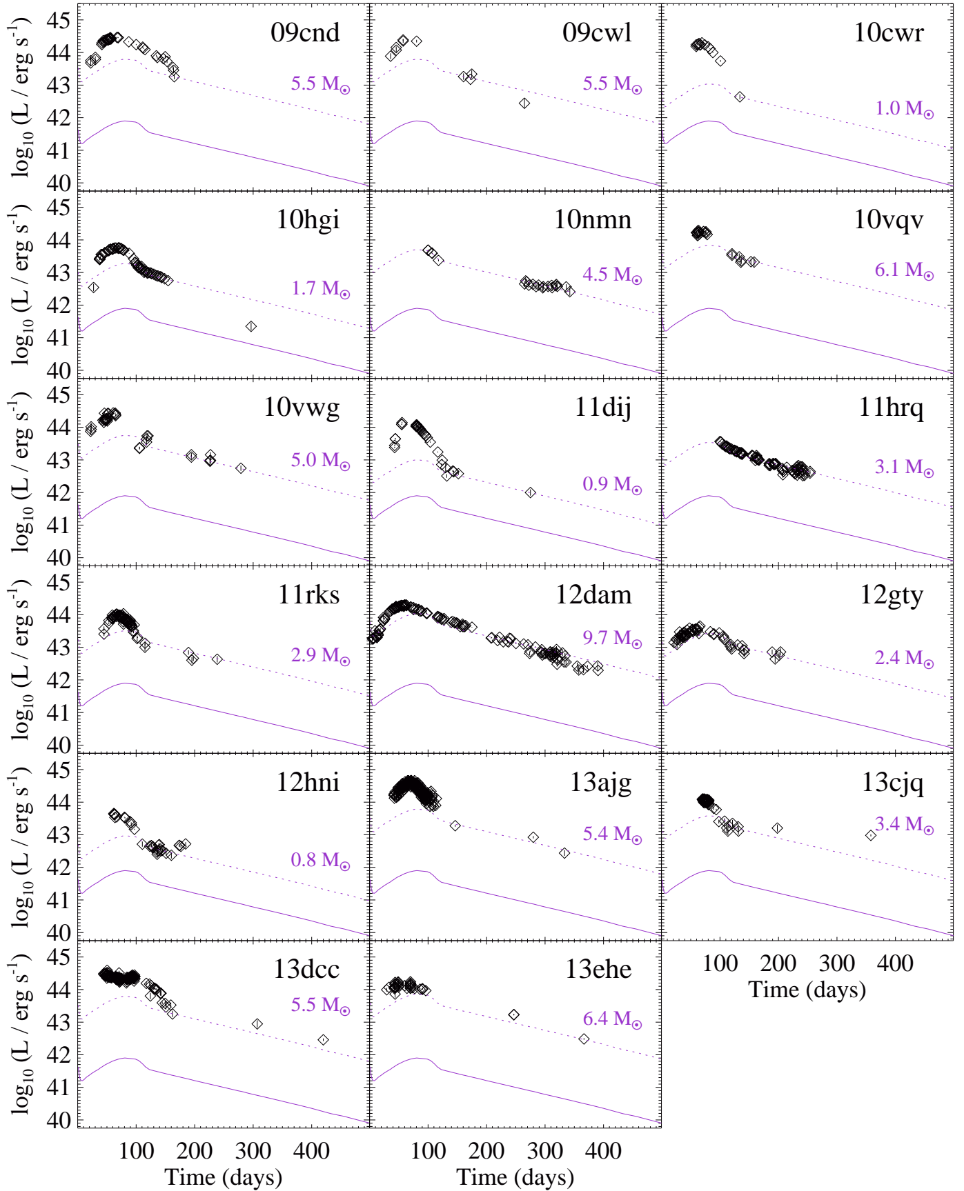
Figure 10. The bolometric light curve of SN 1987A (solid curve) is scaled (dashed curves) to match the decay of SLSNe-I (black diamonds) at late times, after bolometric correction. The M_{\text{Ni}} roughly estimated from this comparison are labelled. The time reference is in restframe days after explosion.
