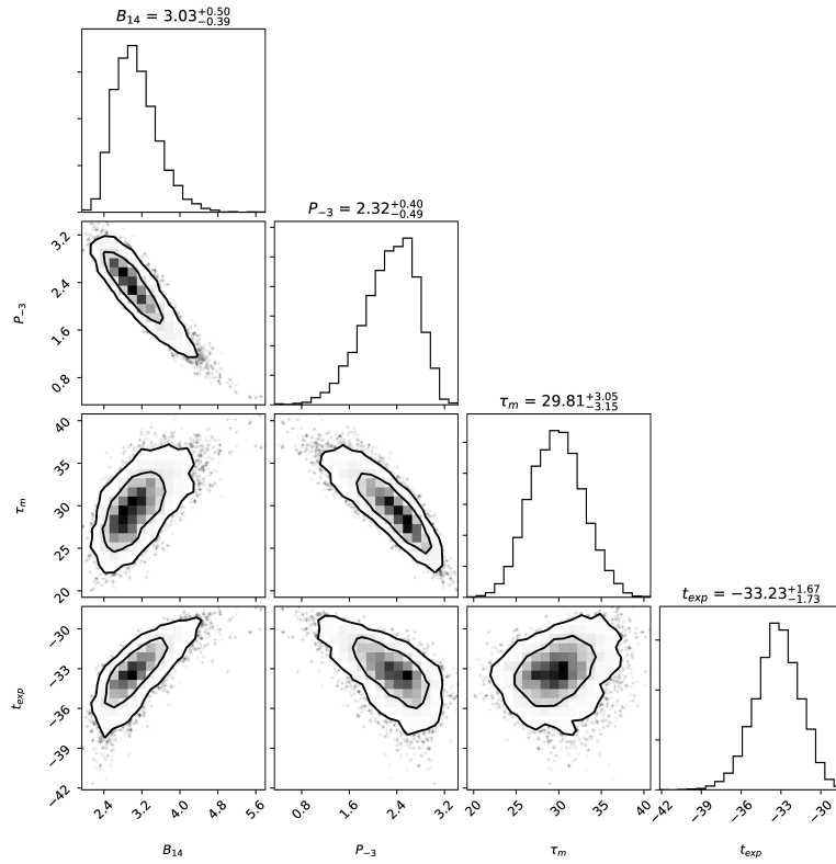
Figure B25. Confidence levels of the best-fit parameters for the magnetar model of PTF 10vwg.
