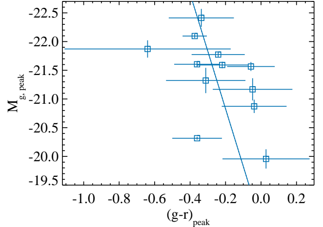
Figure 17. The rest-frame g peak magnitude versus the rest-frame g - r colour at peak, for PTF SLSNe. The solid line shows a linear fit to the data. The Pearson correlation coefficient is r = 0.5 .
