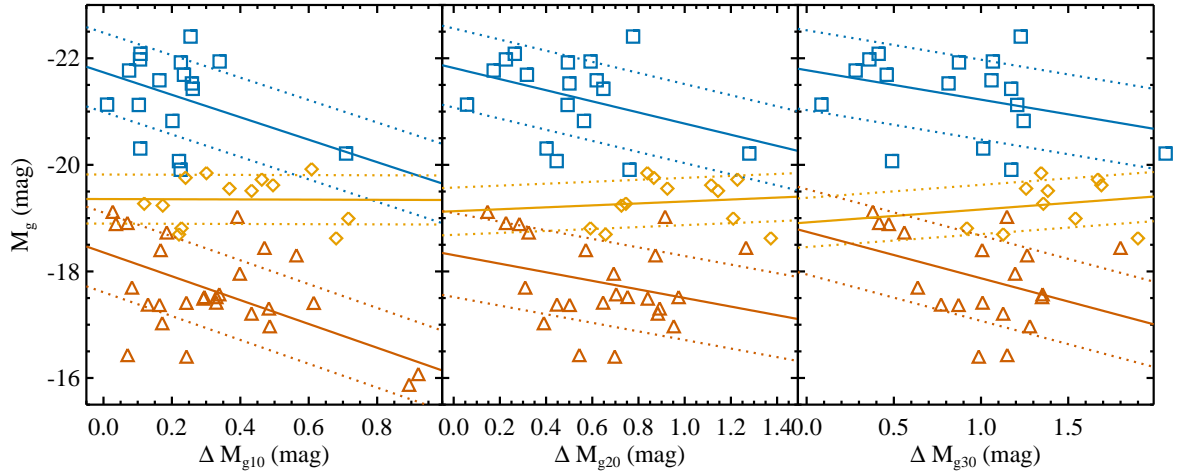
Figure 16. Rest-frame g magnitude at peak and its decay from the peak after 10 (left), 20 (middle), and 30 days (right panel). Blue squares show SLSNe-I, gold diamonds show Ic-BL SNe, and orange triangles Ic SNe, all from PTF. The solid and dotted lines show linear fits through the data, and the intrinsic scatter, respectively.
