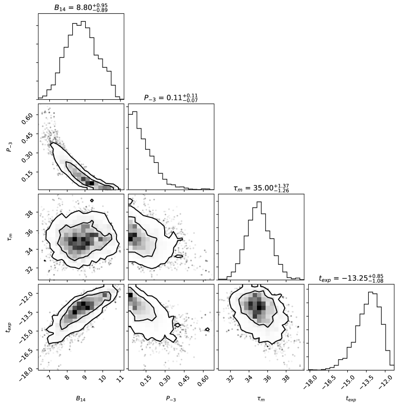
Figure B21. Confidence levels of the best-fit parameters for the magnetar model of PTF 10cwr.
