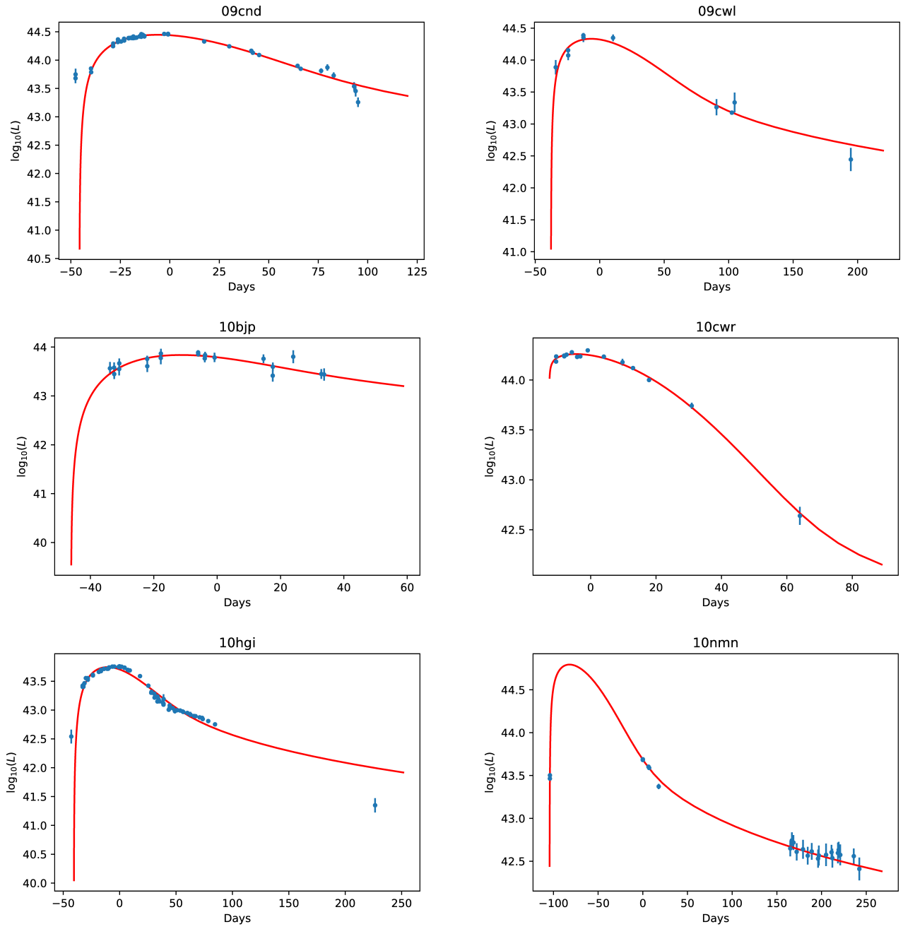
Figure B16. Magnetar fit to the bolometric light curves.
