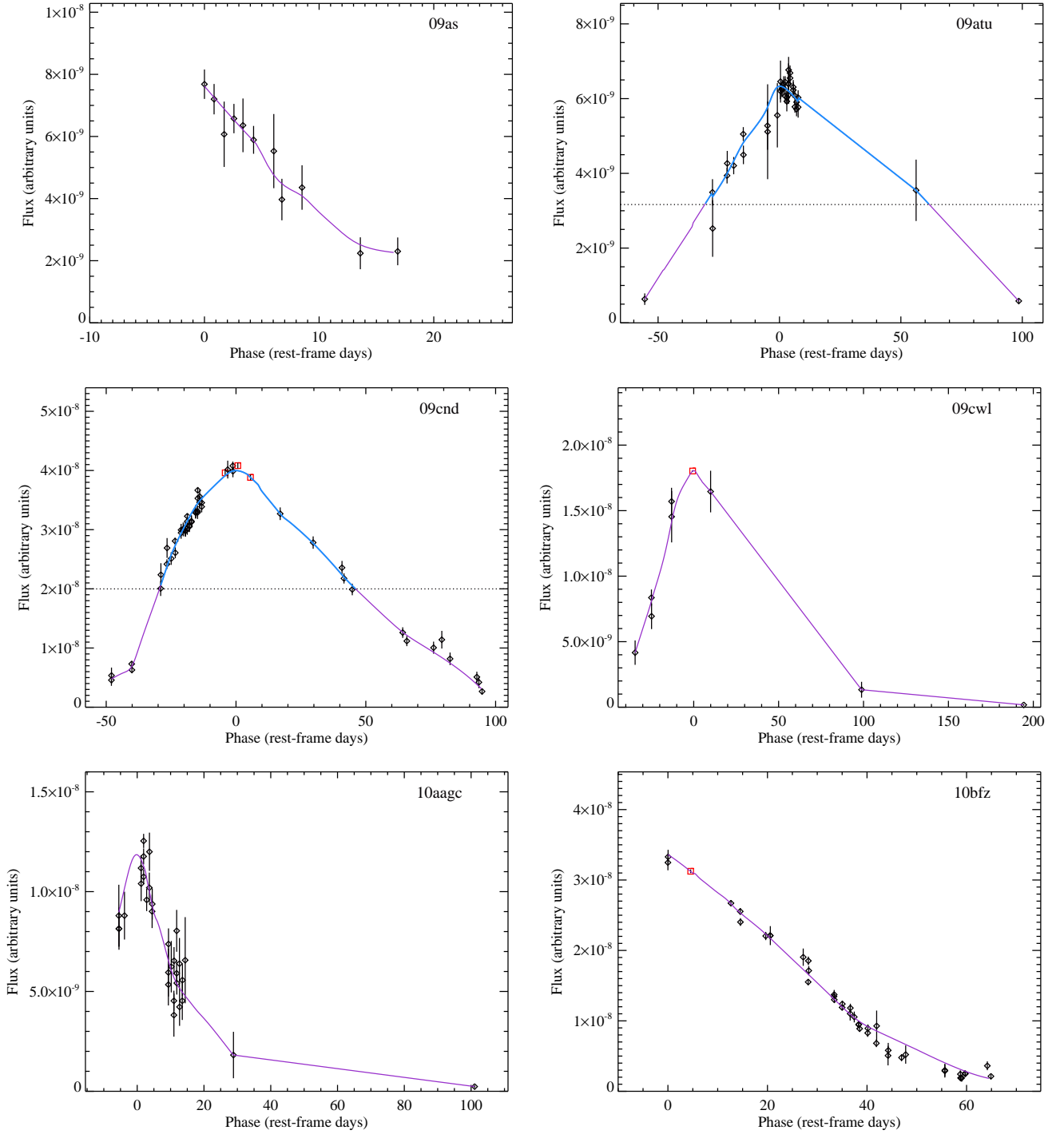
Figure B6. The rest-frame g -band light curves of the SLSNe-I in flux (black diamonds). The smoothed light curves (described in Sect. 4.3) are shown by the solid curves. The red squares indicate the auxiliary points introduced for the light curve smoothing. The horizontal dotted line marks the half-flux limit, which is used to calculate the t_{\text{rise},1/2} and t_{\text{fall},1/2} timescales (Sect. 5.4), when the light curve is well characterized between the half-flux limit and the peak (highlighted blue solid curves).
