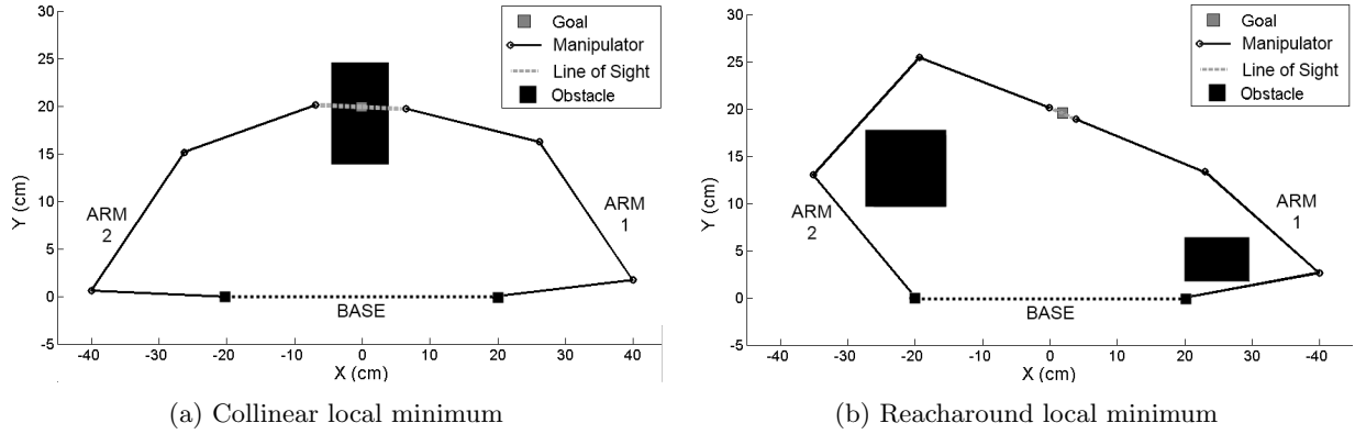
Figure 11: Local Minimum issues with APF approach
