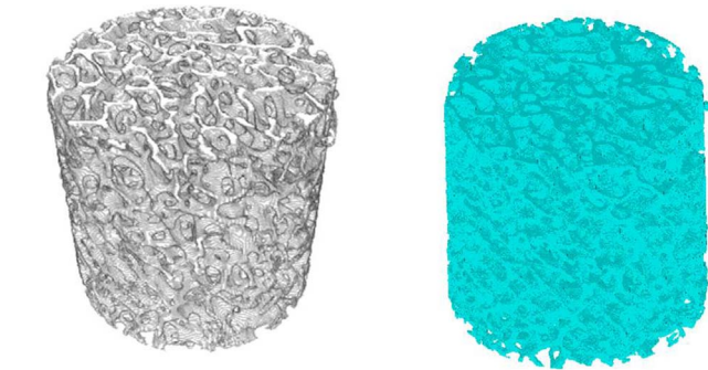
Fig. 3. 3D representation of microCT (left) of Specimen3 and the corresponding microFE model (right).
