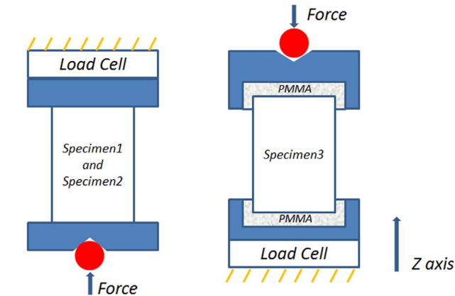
Fig. 2. Scheme of the loading jigs used for testing Specimen1 and Specimen2 (left) and Specimen3 (right).
