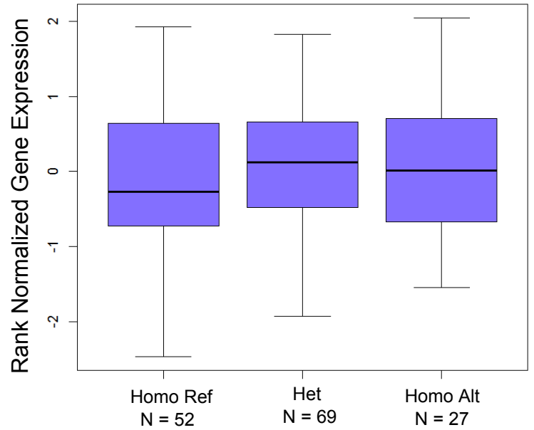
GATA4 : rs1004712 2
