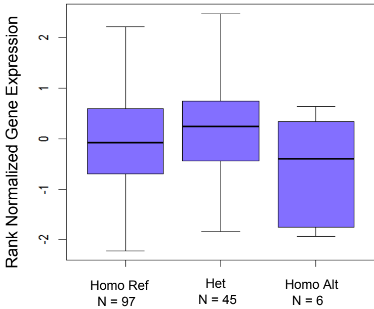
SNAPC5 : rs11629783 2
