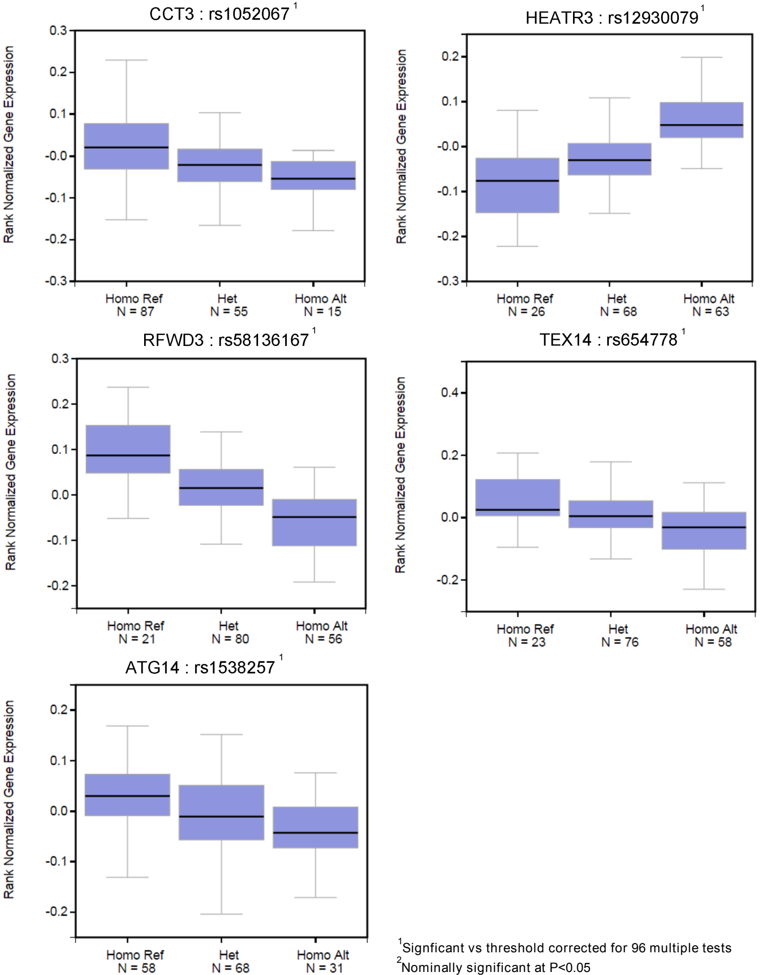
Supplementary Figure 3 - Visualisation of significant eQTL associations. The first five plots are for associations in normal testicular tissue, the remaining six are in TGC tumor tissue. Each plot shows a set of three boxplots of rank-normalised RNA-seq gene expression values for the given gene (Y-axis), split by genotype (X-axis) of the SNP with strongest eQTL association at each risk locus. X-axis indicates the number of individuals for each given genotype.
