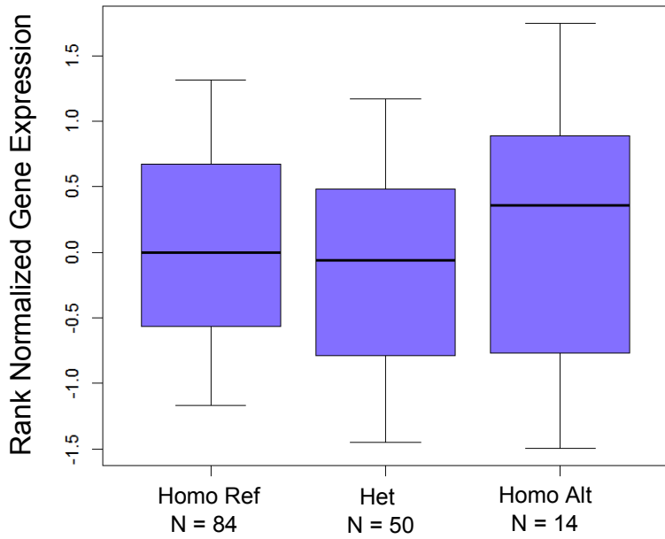
SMARCD1 : rs11629783 2
