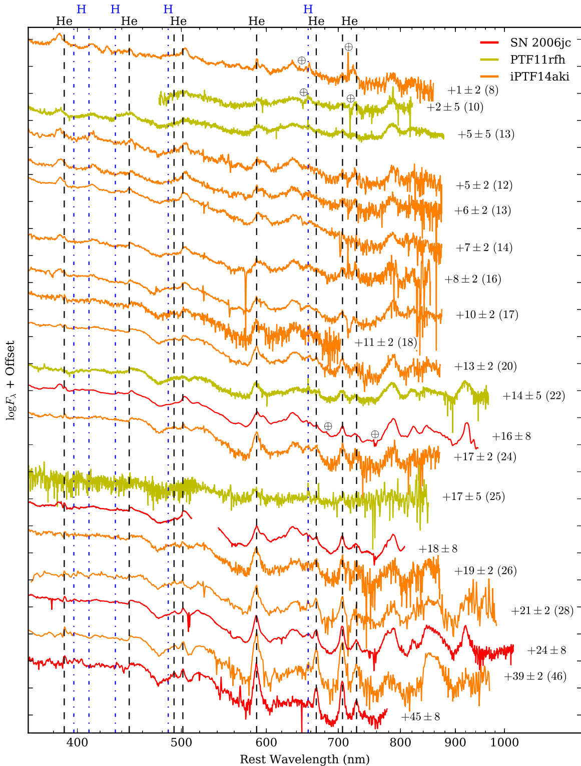
Figure 3. Combined spectral series of PTF11rfl and iPTF14aki with representative spectra of SN 2006jc for comparison. Phase is indicated to the right of each spectrum, with rest-frame days from explosion in parentheses, where available. Vertical lines mark emission wavelengths of various elements, listed along the top axis. The Earth symbol ( \oplus ) marks wavelengths affected by telluric absorption once for each supernova. Tick marks on the vertical axes are 0.5 dex apart. Note the similarity between these three objects and the contrast with the early spectra in Figure 4.
