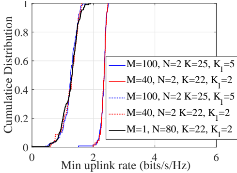
Figure 1. The cumulative distribution of the per-user uplink rate, for ( M = 100, K = 25, K_1 = 5 ) and ( M = 40, K = 22, K_1 = 2 ) with D = 1 km, \tau = 20 , and \text{SINR}_k^t = 1 . The solid curves refer to the proposed Algorithm 1, while the dashed curves present the case u_{mk} = 1, \forall m, k , and solve Problem P_4 .
