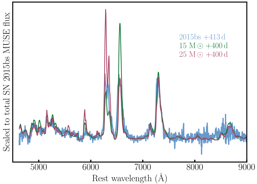
Supplementary Figure 11: Comparison of the nebular spectrum of SN 2015bs with model spectra at similar epochs. The model spectra are produced by progenitors of 15 and 25 M ⊙ at solar metallicity 12 . The spectra are scaled to the total flux contained within the MUSE wavelength range of the SN 2015bs spectrum.
