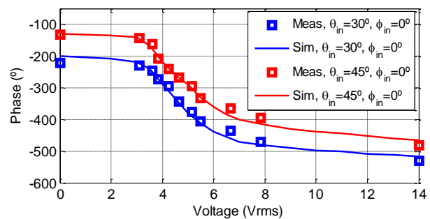
Fig. 4 Phase of the reflection coefficient (100 GHz) of the cells as a function of the rms voltage at two angles of incidence for the case where the bias signal applied to the LC is 0.33 Hz-square.
