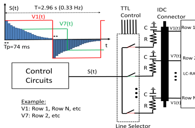
Fig. 3 Schematic of the retention circuits that maintain a fixed voltage applied to the LC together with the applied signals.
