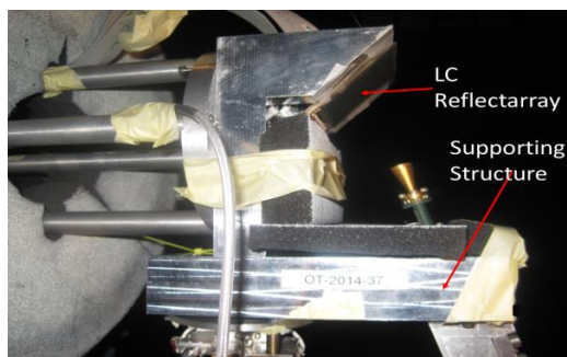
Fig. 5 Photograph of the single offset LC based reflectarray antenna
