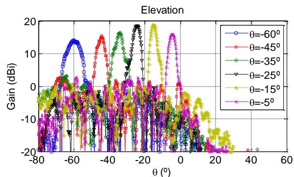
Fig. 6 Measured elevation radiation patterns at 100 GHz of several scan angles
