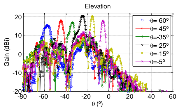
Fig. 8 Measured elevation radiation patterns at 104 GHz of several scan angles
