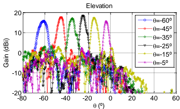
Fig. 7 Measured elevation radiation patterns at 96 GHz of several scan angles
