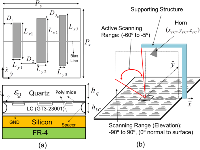
Fig. 1 Schematic of the LC-reflectarray. (a) Cells showing its different parts, (b) antenna configuration. Dimensions of the cells (mm): P_y=1.145 , P_x=1.093 , L_{x1}=0.707 , L_{x2}=0.748 , L_{x3}=0.792 , L_{y1}=0.20 , L_{y2}=0.211 , L_{y3}=0.20 , D_1=0.171 , D_2=0.096 , D_3=0.042 , h_q=550 , h_{LC}=0.075 .
