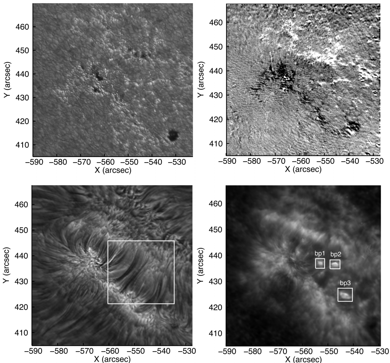
Fig. 1. Simultaneous ROSA images of the G band ( top left ), line-of-sight magnetogram ( top right ), H\alpha core ( bottom left ), and Ca\ II\ K core ( bottom right ). The magnetogram colour scale is in Gauss, where white indicates positive magnetic polarities, while black demonstrates polarities which are negative. Artificial saturation at \pm 400 G is implemented to highlight regions of weak magnetic polarity on the solar surface. The white rectangle in the H\alpha core image indicates the approximate position where most of the jets are observed. White rectangles in the Ca\ II\ K image, identified by “bp1”, “bp2”, and “bp3”, are the bright points selected for temporal analysis. Axes are in heliocentric arcseconds, where 1'' \approx 725 km.
