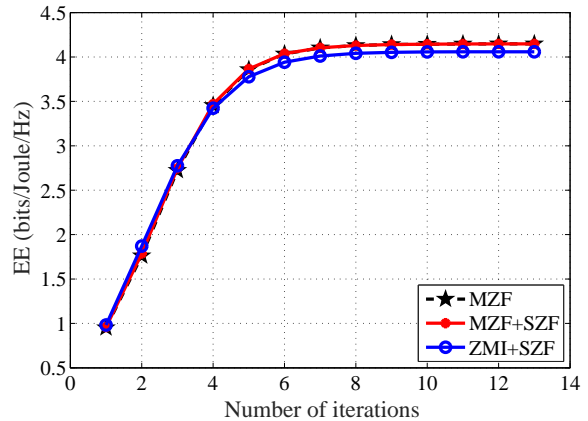
Fig. 3: The convergence vs. iteration number under N_M = 64 and QoS \bar{r}_k = \bar{r}_{(s,\ell)} \equiv 4 Mbps.
