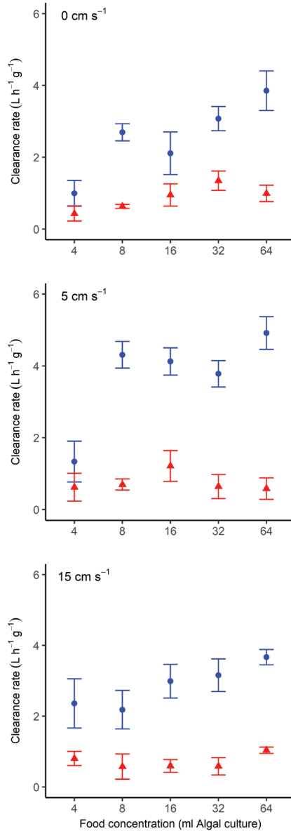
Figure 1. Clearance rates of the native mussel, Mytilus edulis (blue circles), and invasive Pacific oyster, Crassostrea gigas (red triangles), as a function of algal food concentration at flow velocities of 0, 5 and 15 cm s -1 .
