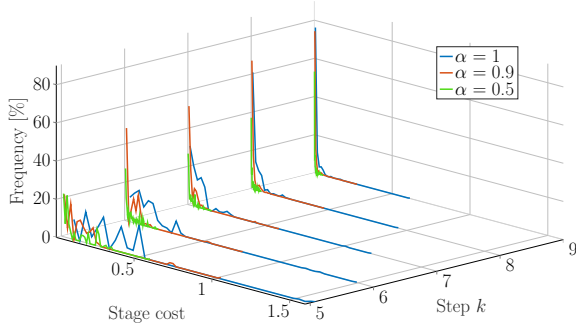
Fig. 3. Distribution of \ell(x_k, u_k, i_k) estimated using 1000 randomly generated switching sequences. The cost of trajectories corresponding to higher \alpha values are more spread out compared to \alpha = 0.5 and have a noticeably longer right tail.
