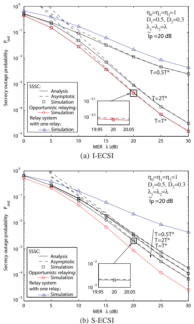
Fig. 2. Secrecy outage probability versus MER.
