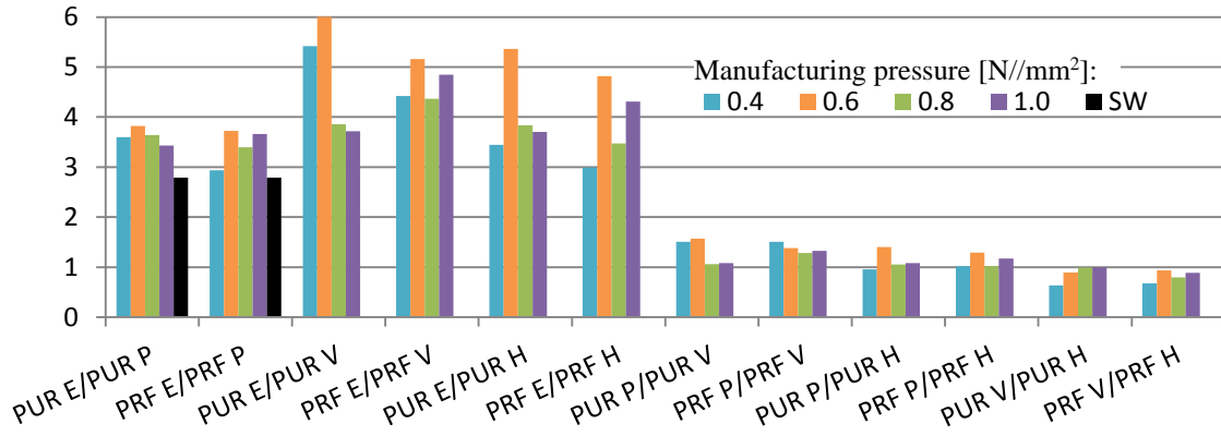
Figure 7 Ratios of 5-percentile shear strength values for different manufacturing pressures
