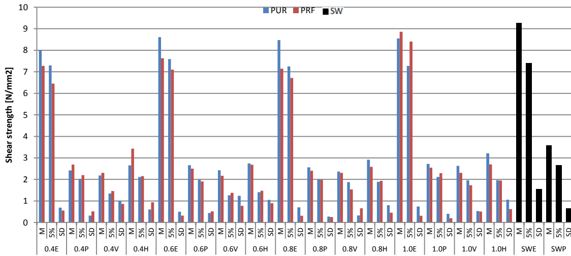
Figure 3 Shear strength values †
