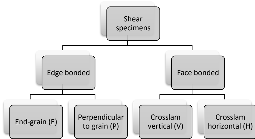
Figure 1 Schema of specimen configurations for shear tests
