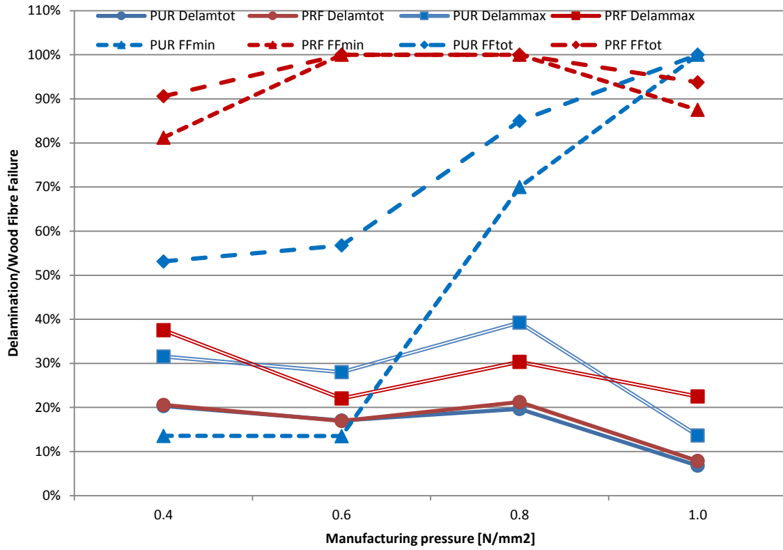
Figure 9 Median delamination and wood fibre failures values for specimens manufactured with different pressures
