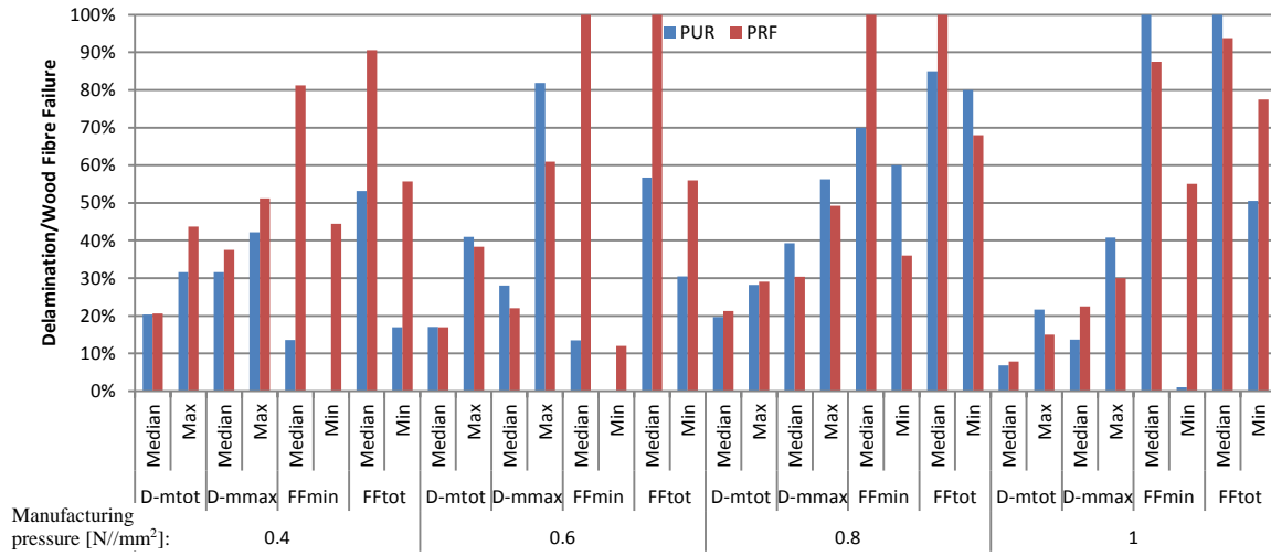
Figure 4 Delamination tests results ‡
