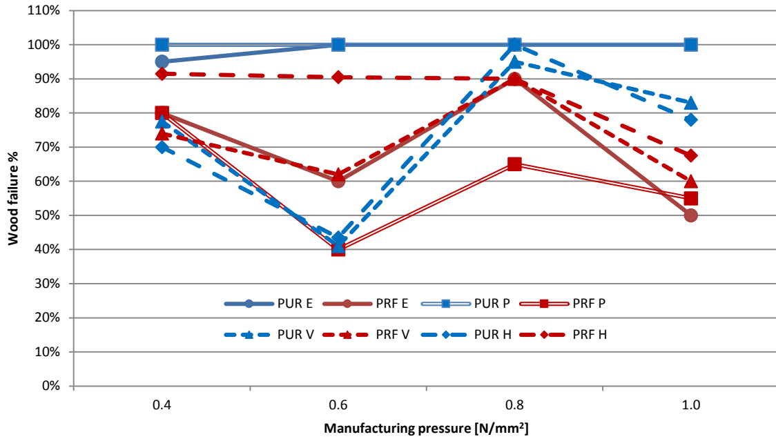
Figure 6 Median wood failure percentage values for different configurations of specimens manufactured with different pressures
