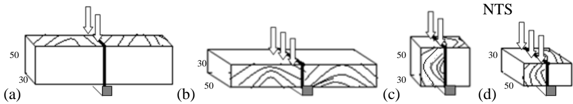
Figure 2 Shear test specimens for: end-grain (a), perpendicular to grain (b) loading, and crosslam bonded elements vertically (c) and horizontally (d) loaded (dimensions in mm)
