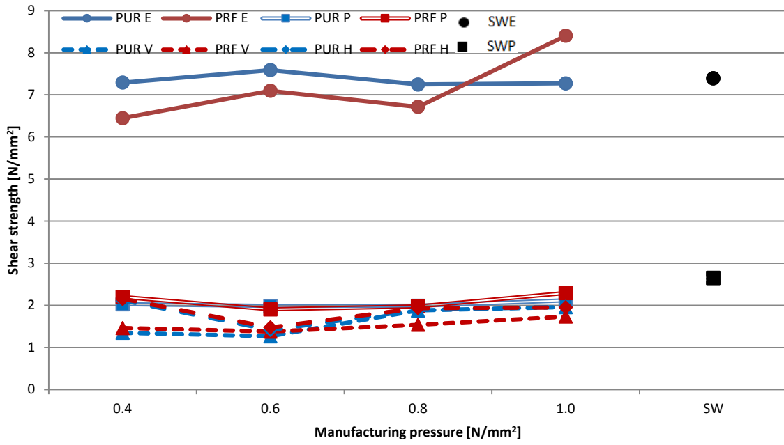
Figure 5 5-percentile shear strength values for different test configurations
