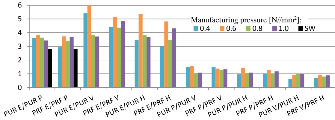
Figure 7 Ratios of 5-percentile shear strength values for different manufacturing pressures
