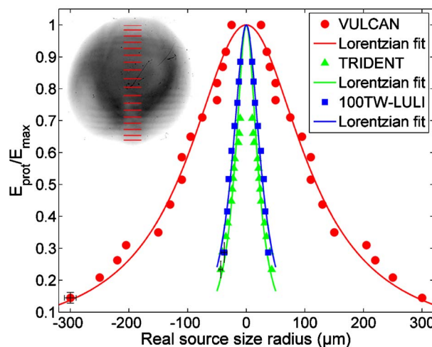
FIG. 7. (Color online) Energy resolved, real source size of the laser-accelerated proton beams. The energies are normalized to the maximum proton energy of each shot. A Lorentzian fit (line) can be applied with a FWHM of 240 \mu\text{m} for VULCAN, 44 \mu\text{m} for TRIDENT, and 56 \mu\text{m} for 100TW-LULI. Inset: intensity modulation in a RCF for E_{\text{prot}} > 8.5 MeV. The positions of the imprinted lines are marked in red. For the measurement error of the line counting to estimate the source size of the proton beam a double line spacing is sufficient: TRIDENT 6 \mu\text{m} , 100TW-LULI 10 \mu\text{m} , VULCAN 20 \mu\text{m} . See example error bars for the lower left data points.
