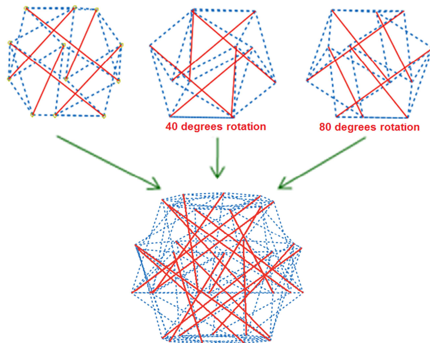
Figure 1 (B) The formation of nucleoskeletal network. The same method shown in Figure 1 (A) applies to 3 sets round-configuration tensegrity structures, with nuclear lamina and chromatin modelled by struts and cables, respectively.
