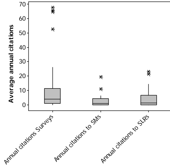
Figure 10: Box-plots of average normalized citations to regular surveys, SMs and SLRs
