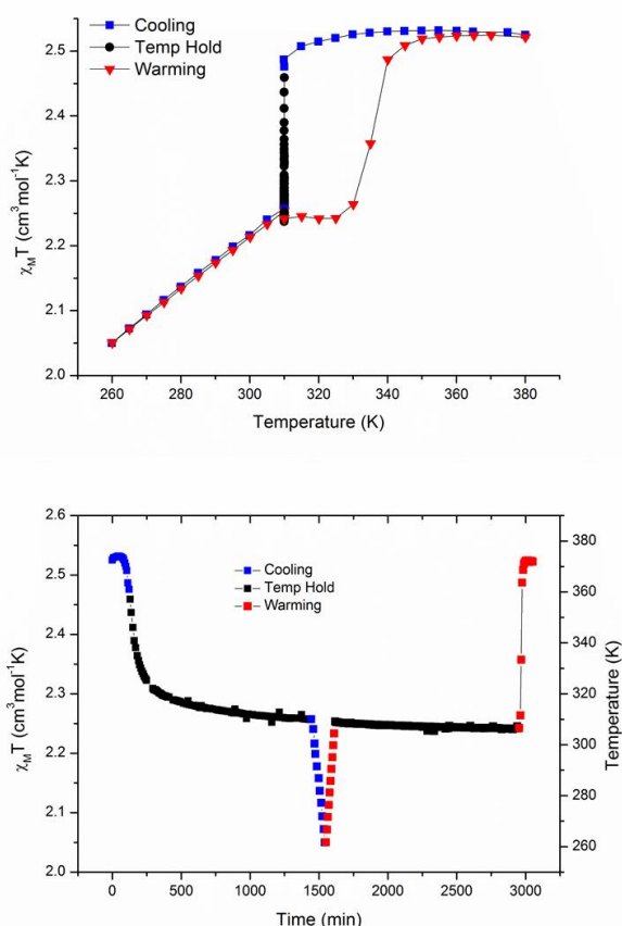
Fig. 6. a) \chi_m T v T plot for complex (1) highlighting the time dependence of the spin state at fixed temperature; b) Plots of \chi_m T v time and T v time for complex (1).
