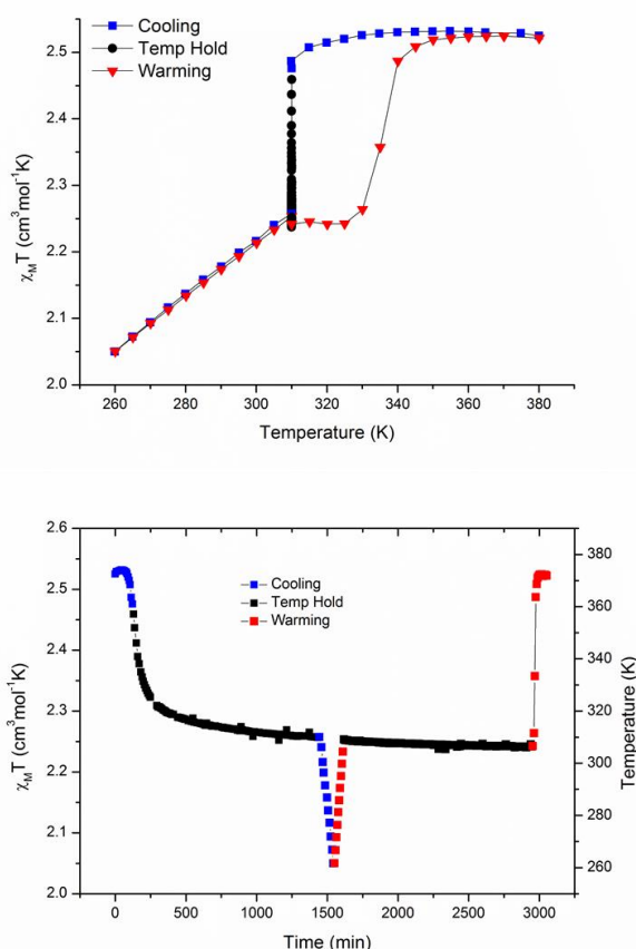
Fig. 6. a) \chi_m T v T plot for complex (1) highlighting the time dependence of the spin state at fixed temperature; b) Plots of \chi_m T v time and T vs time for complex (1).
