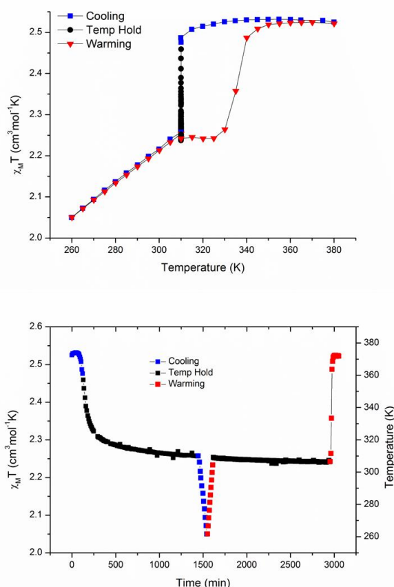
Fig. 6. a) \chi_m T vs T plot for complex (1) highlighting the time dependence of the spin state at fixed temperature; b) Plots of \chi_m T vs time and T vs time for complex (1).
