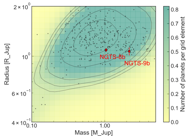
Figure 8. Shows NGTS-8b and NGTS-9b in the planetary radius vs planetary mass plot, in regards with all exoplanets from the NASA Exoplanet Archive with radius uncertainty below 10% or mass uncertainty below 50% and with an incident flux received by the planets greater than 2 \times 10^5 \text{ W m}^{-2} . The background and the dotted black lines represents the point density per grid element.
