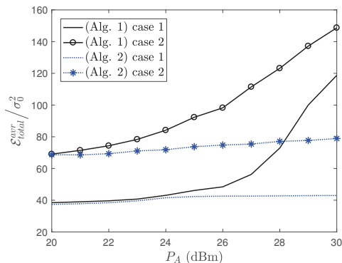
Fig. 8. The ratio of total harvested energy \mathcal{E}_{\text{total}}^{\text{avr}} to \sigma_0^2 as a function of the parameter P_A . Two sub-cases are considered. In the first sub-case, we set \{\sigma^2, \tilde{\sigma}^2\} = \{-2, 0\} dBm. The second sub-case, we set \{\sigma^2, \tilde{\sigma}^2\} = \{-2, 3\} dBm. Other system parameters: N = 7 and K = 3 .
