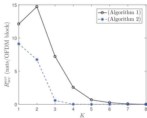
Fig. 5. The achievable secrecy rate R_{\text{sec}}^{\text{avr}} as a function of the parameter K . Other system parameters: N = 8 and \{P_A, \sigma^2, \tilde{\sigma}^2\} = \{30, 10, 10\} dBm.
