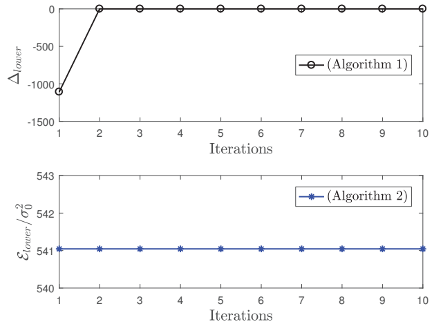
Fig. 2. The convergence rate of the proposed algorithms. Other parameters: N = 10 , K = 2 , and \{P_A, \sigma^2, \bar{\sigma}^2\} = \{30, 10, 10\} dBm.
