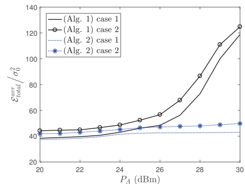
Fig. 10. The ratio of total harvested energy \mathcal{E}_{\text{total}}^{\text{avr}} to \sigma_0^2 as a function of the parameter P_A . Two sub-cases are considered. In the first sub-case, we set \{\sigma^2, \tilde{\sigma}^2\} = \{-2, 0\} dBm. The second sub-case, we set \{\sigma^2, \tilde{\sigma}^2\} = \{2, 0\} dBm. Other system parameters: N = 7 and K = 3 .
