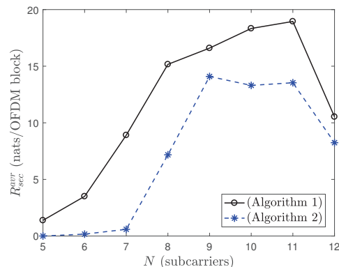
Fig. 3. The achievable secrecy rate R_{\text{sec}} as a function of the number of subcarriers N . Other system parameters: K = 2 and \{P_A, \sigma^2, \bar{\sigma}^2\} = \{30, 10, 10\} dBm.
