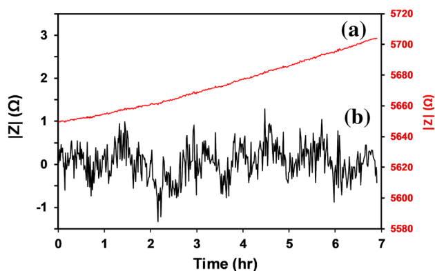
Fig. 5 Time variation in |Z| for 9.1 mM NaOH solution ( \sim 200 \text{ mS m}^{-1} ) for a raw data, and b drift-corrected data, using a fourth order polynomial fit. The drift-corrected data gives an rms noise of 0.39 \Omega
