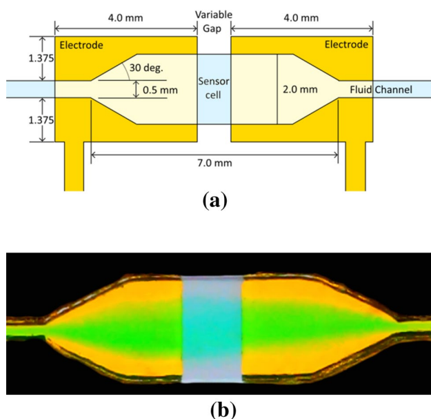
Fig. 1 a Electrode pair and sensor cell schematic. b Photo of Au/Ti electrode pair and sensor cell with green dye input, through DI water prefill. A modest excess flow volume is required to totally clear the cell of previous sample contents. Dimensions are as in (a)
