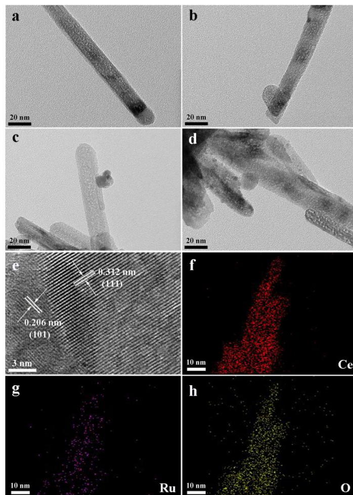
Fig. 3. TEM images of reduced catalysts \text{CeO}_2 (a), 2.5\text{Ru}/\text{CeO}_2 (b), 5\text{Ru}/\text{CeO}_2 (c) and 10\text{Ru}/\text{CeO}_2 (d). HRTEM (e) and element mapping (f-h) of reduced 5\text{Ru}/\text{CeO}_2 .
