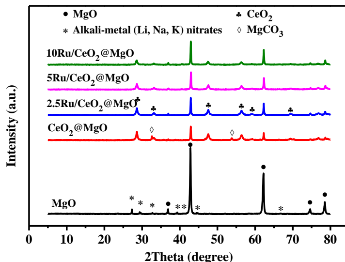
Fig. 8. XRD patterns of MgO and spent DFMs ( \text{CeO}_2\text{-MgO} is after 2 ICCU cycles and others are after 10 ICCU cycles).
