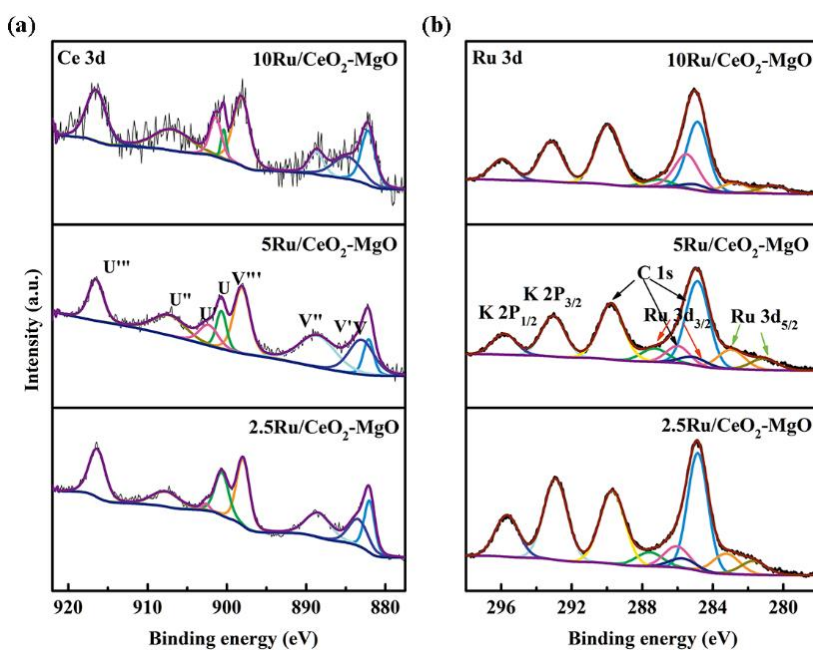
Fig. 10. XPS spectra and peak fitting curves: Ce 3d (a) and Ru 3d (b) of spent DFMs after 10 cycles of ICCU process.
