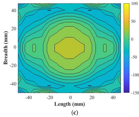
Figure 2. (a) Phase values above RCA in \phi_{RP1}(x,y) (b), phase values in \phi_{RP2}(x,y) before correction, and (c) modulated phase values in \phi_{RP2}(x,y) after correction.
