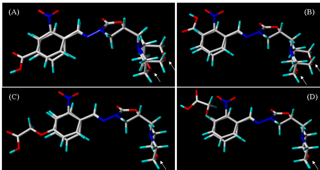
Fig. 2. The overlap of NPAMOZ and four immunizing haptens based on the lowest energy conformations. (A) NPAMOZ and hapten 1; (B) NPAMOZ and hapten 2; (3) NPAMOZ and hapten 3; (4) NPAMOZ and hapten 4. The arrows point at the morpholine ring, the conformation of which was changed after introducing of different spacers.
