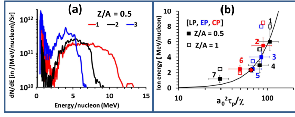
FIG. 2 (color online). (a) Graph showing comparison between three ion ( Z/A = 0.5 ) spectra, where the position of the spectral peaks is plotted in (b) as a function of a_0^2 \tau_p / \chi . The experimental parameter set [ a_0 , target material, target thickness ( \mu\text{m} )] for the data points 1–7 is [15.5, Cu, 0.1], [10, Cu, 0.05], [13.8, Cu, 0.1], [7.5, Al, 0.1], [6.9, Al, 0.1], [13.6, Al, 0.5], and [14.1, Al, 0.8], respectively. The black solid line in (b) represents the ion energy estimated from the analytical modeling described in the text. The red circle represents the data from Henig et al. in Ref. [15].
