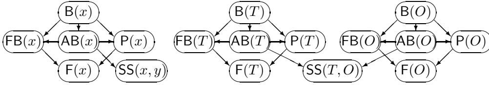
Fig. 3. Left: graph \mathcal{G} in Example 13. Right: propositionalized PPL network in Example 13. Nodes contain only capital letters of relations and individuals.
