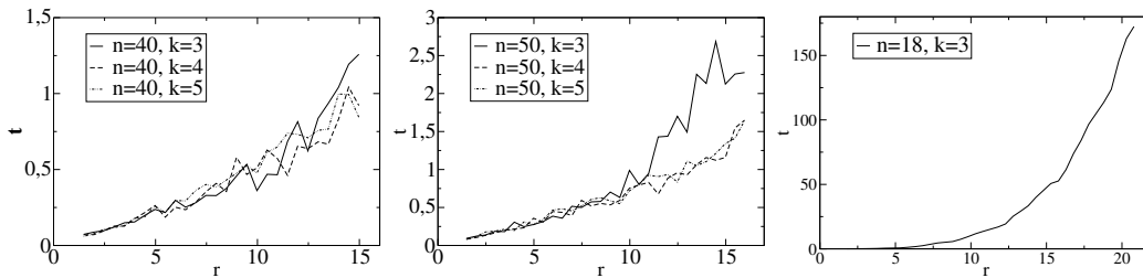
Fig. 1. Left and middle: time (seconds) to check satisfiability of random problems. Right: time (seconds) to check satisfiability of satisfiable random problems (note that these problems required more effort).
