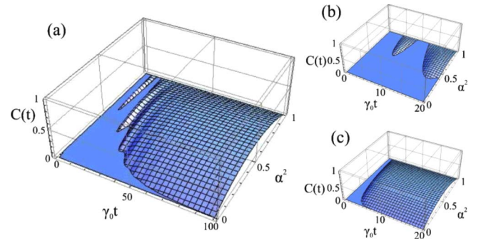
FIG. 2. (Color online) (a) Concurrence as a function of time and \alpha^2 for two atoms prepared in factorized state (10) and interacting with a common Lorentzian structured reservoir. For comparison we show the short-time region of (a) in (b), and the Markovian common reservoir result in (c).
