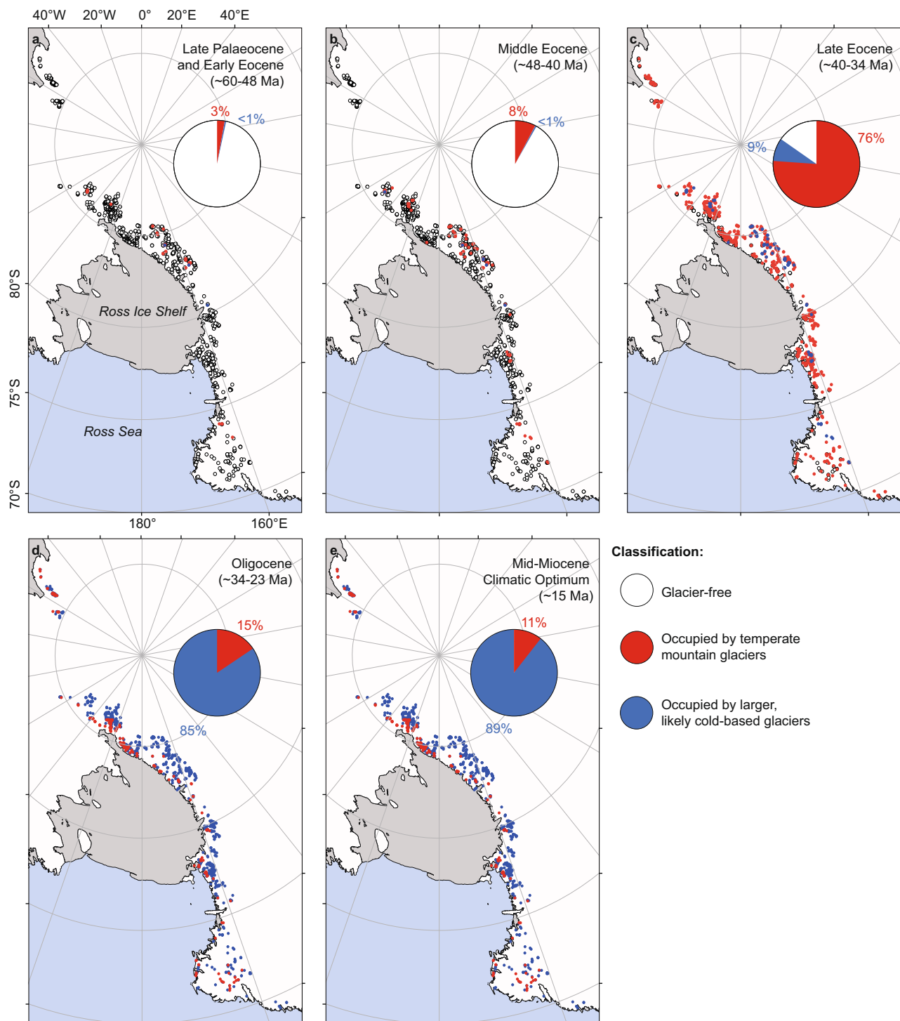
Fig. 2 | Glacier-free cirques in the Transantarctic Mountains are classified according to their glacial status during various periods of the Cenozoic. a–e Pie charts show the percentage of cirques classified as glacier free (white), occupied by temperate mountain glaciers (red %), and occupied by larger, likely cold-based
