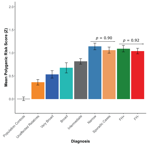
Fig. 1 Mean Leave-N-Out PGC3-SCZ PRS for each of the diagnostic categories in the ISHDSF sample, sporadic SCZ cases and ancestry-matched population controls. A subset of sporadic cases with family history (FH) information are further divided into FH+ (green bar) and FH- (red bar) categories. Unaffected relatives (dark orange bar) are distinct from population controls (black bar) as they represent unaffected individuals in the families. Familial SCZ cases are represented in the narrow spectrum category as described in the methods section. Error bars represent the standard error of the observed mean. X axis shows each of the diagnostic categories. Y axis shows the mean normalized Z-score for PGC3-SCZ.
