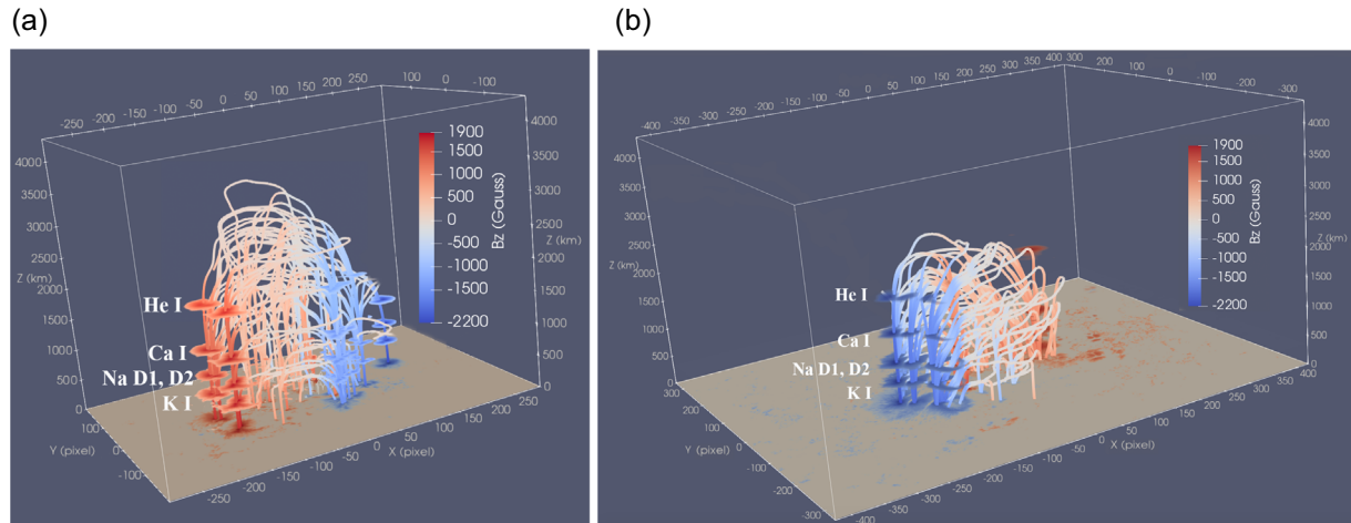
Fig. 4. The figure illustrates the three-dimensional magnetic field of (a) AR 11166 (left) and (b) 12192 (right). The red-blue colour bar refers to the positive-negative polarity vertical B_z magnetic field values measured at the solar surface and computed as function of heights in the solar atmosphere. Particular heights outlining approximately the heights of the line formation of K I, Na D, Ca I, and He I are highlighted.
