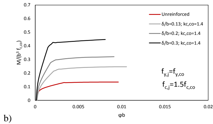
Figure 19. Normalised moment-curvature curves for jacketed sections ( \rho_j = 2\% , \rho_{co} = 1\% , n = 0.25 ); a) f_{y,j} = f_{y,co} ; f_{c,j} = f_{c,co} . b) f_{y,j} = f_{y,co} ; f_{c,j} = 1.5 f_{c,co} .
